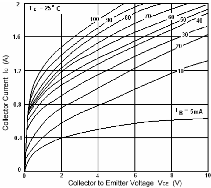
Fig.3 Static Characteristic
