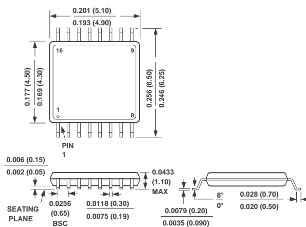
Figure 29. 16-Thin Shrink Small Outline Package [TSSOP] (RU-16)
