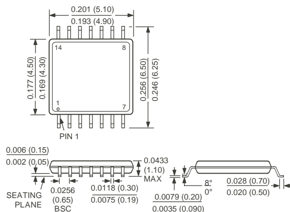
Figure 28. 14-Thin Shrink Small Outline Package [TSSOP] (RU-14)
