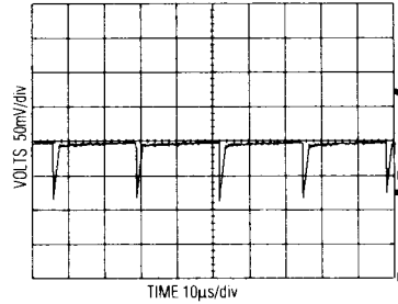
REGULATOR 7 V OUT = -30V WITH 150kΩ LOAD
