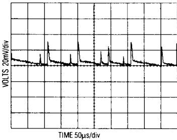
REGULATOR 8 V OUT = +15V WITH 1.5kΩ LOAD
