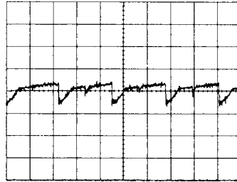
REGULATOR 6 V OUT = -5V WITH 250kΩ LOAD
