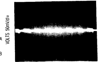
TIME 100μs/div
