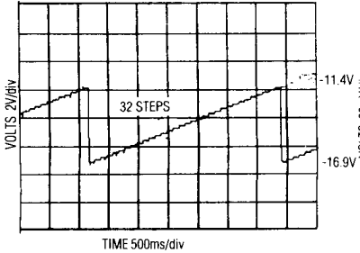
REGULATOR 7 V OUT = -11.4 TO -16.9 V WITH 10kΩ LOAD
