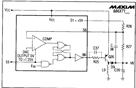
Figure 4. Functional Diagram and Circuit for DC-DC Converter V6
