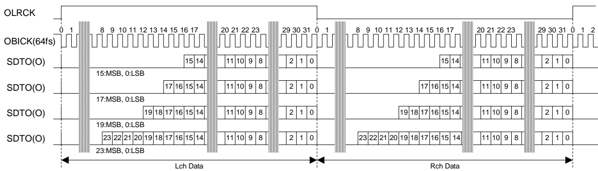
Figure 7. LSB Timing
