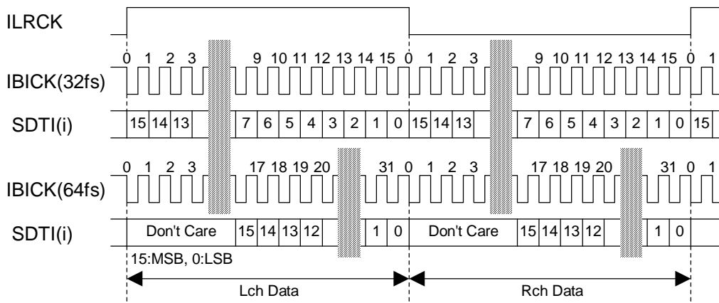
Figure 2. Mode 0 Timing
