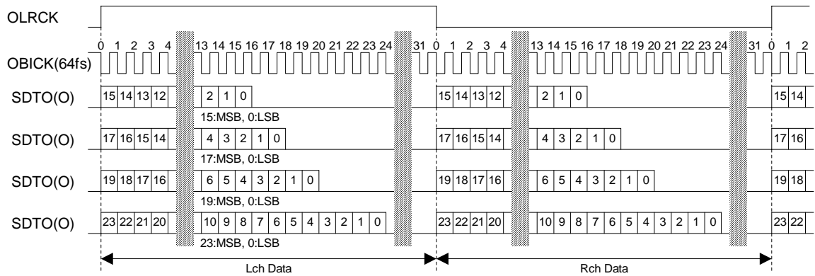
Figure 8. MSB Timing
