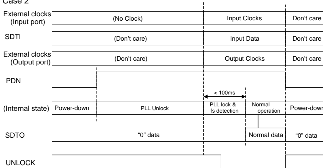
Figure 13. System Reset 2
