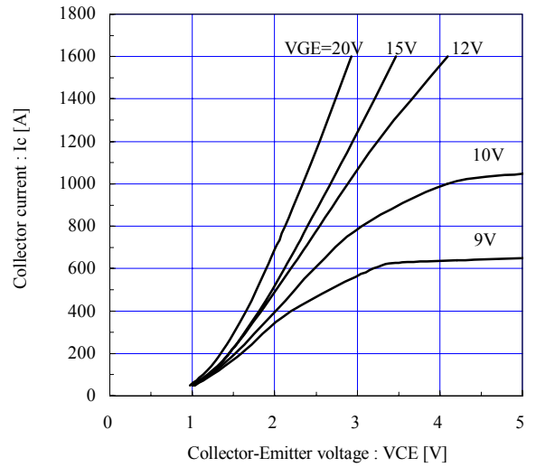
Collector current vs. Collector-Emittor voltage (typ.) Tj= 125°C, sense terminal
