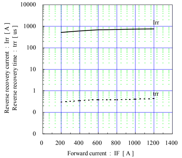
Reverse recovery characteristics (typ.) Vcc=900V, VGE=±15V, Rg=1.0Ω, Tj=125°C
