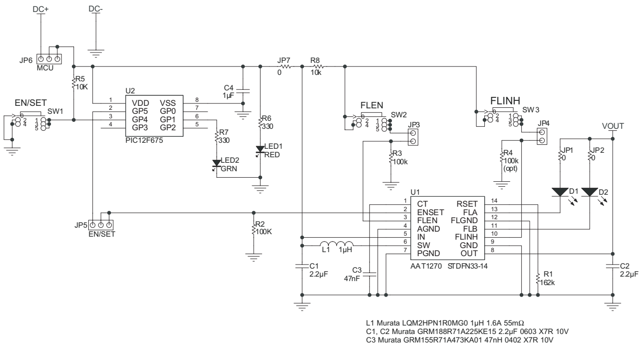
Figure 3: AAT1270 Evaluation Board Schematic.
