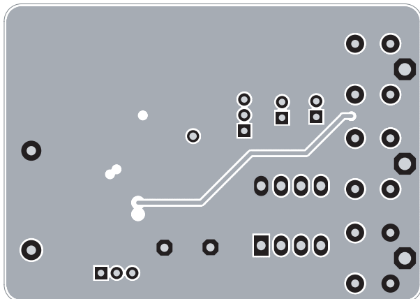
Figure 6: AAT1270 Evaluation Board Third Layer.
