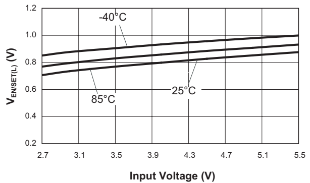
EN/SET, FLEN Input Low Threshold vs. Input Voltage
