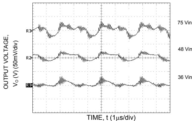
Figure 3. Typical Output Ripple and Noise at Room Temperature, I_o = I_{o,max} , C_{o,ext} = C_{o,min} = 330\mu F .
