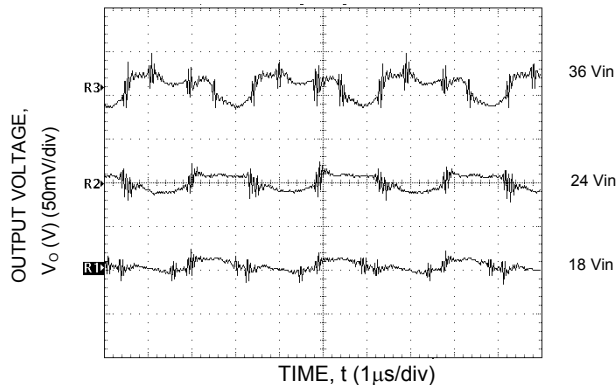
Figure 9. Typical Output Ripple and Noise at Room Temperature, I_o = I_{o,max} , C_{o,ext} = C_{o,min} = 330\mu F .
