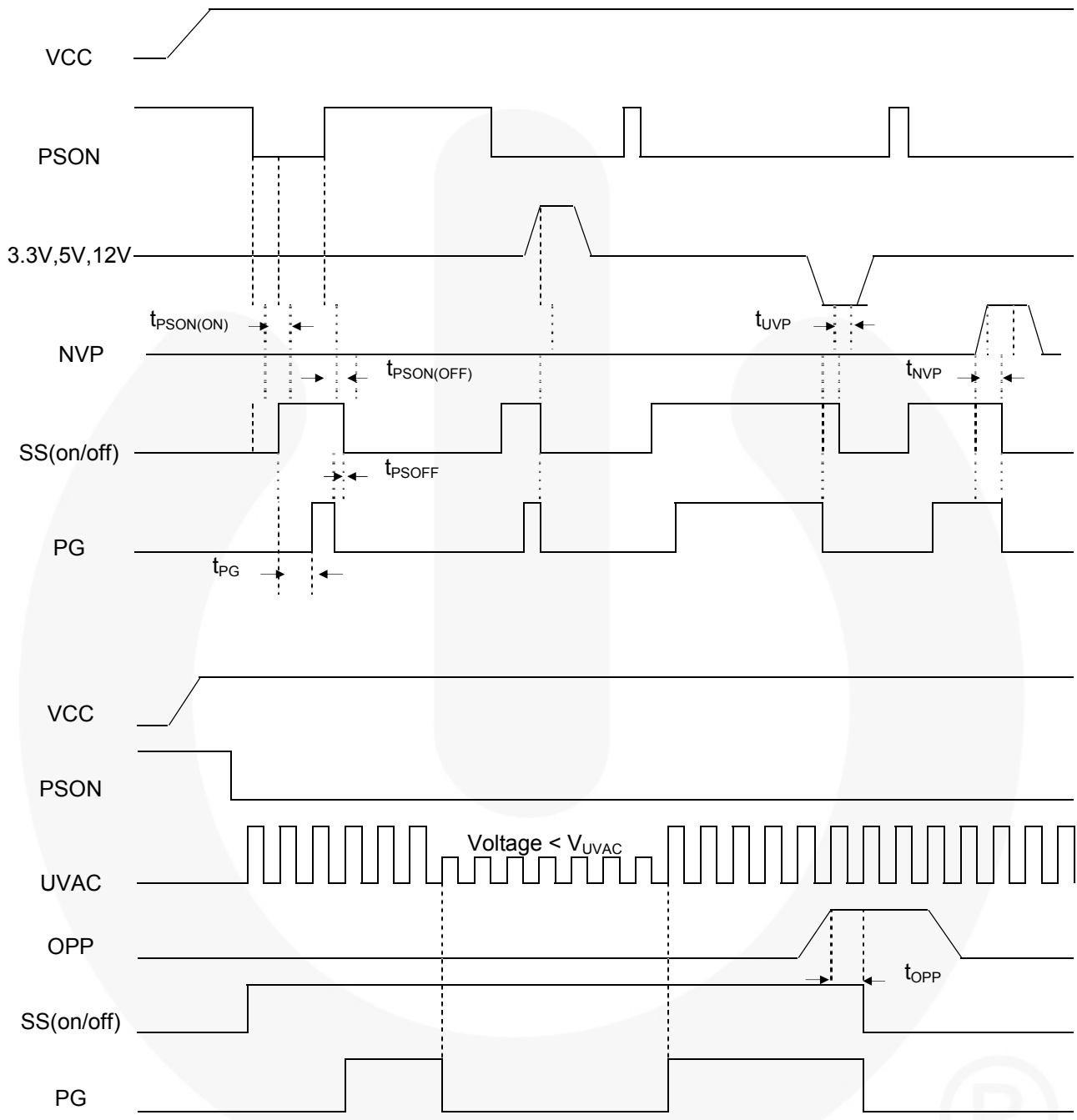
Figure 20. Timing Diagram
