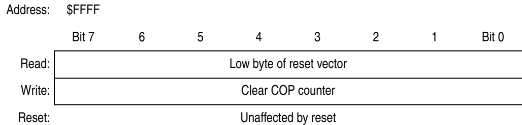
Figure 19-3. COP Control Register (COPCTL)
