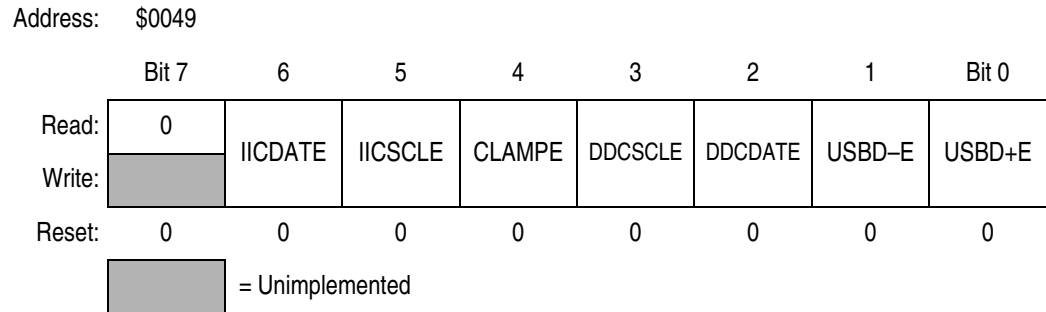
Figure 17-15. Port D Configuration Register (PDCR)
