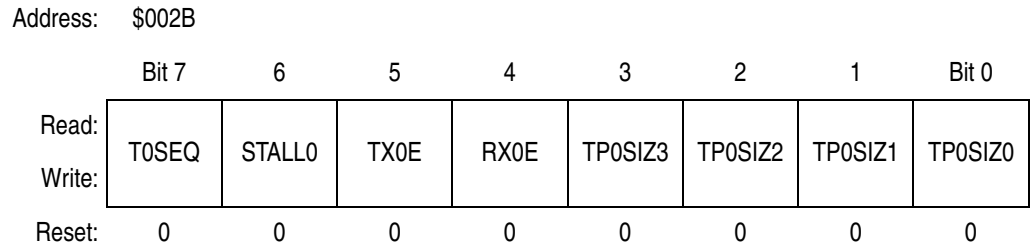
Figure 13-4. USB Control Register 0 (UCR0)
