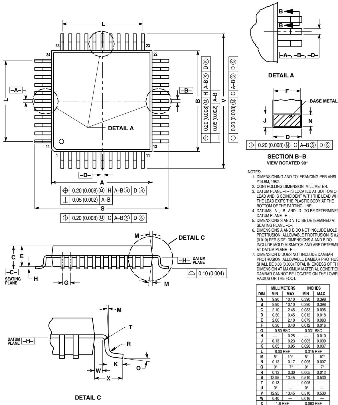
Figure 22-2. 44-Pin QFP (Case #824A)
