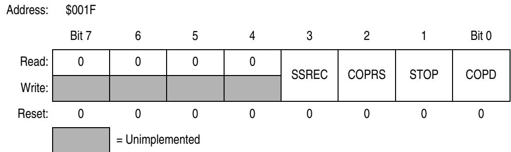
Figure 19-2. Configuration Register 1 (CONFIG1)
