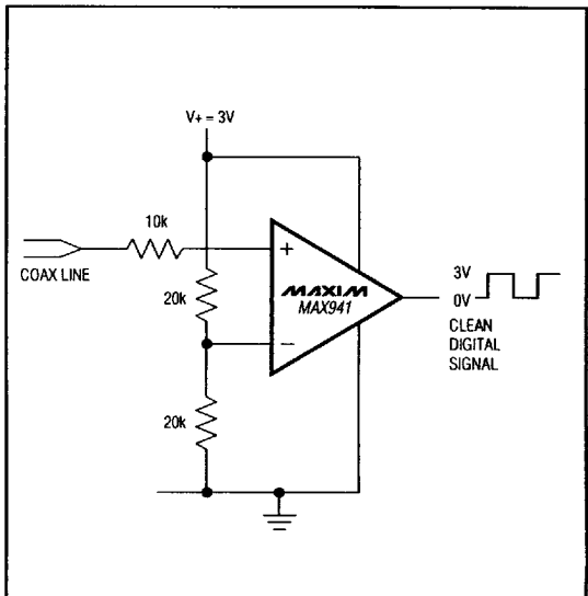
Figure 6 Line Transceiver Application
