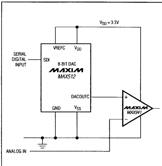
Figure 5 3.3V Digitally Controlled Threshold Detector
