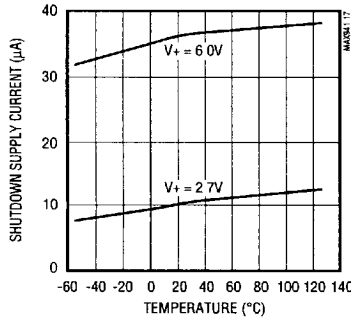
MAX941 SHUTDOWN SUPPLY CURRENT vs. TEMPERATURE
