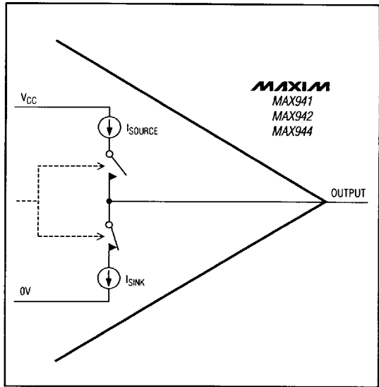
Figure 4 Output Stage Circuitry
