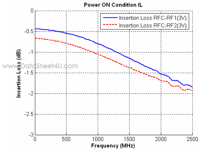
Figure 8. Insertion Loss – Power On
