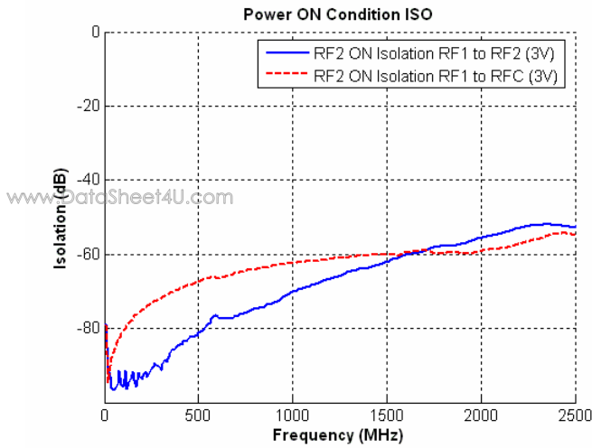
Figure 12. Isolation: RF2 – Power On
