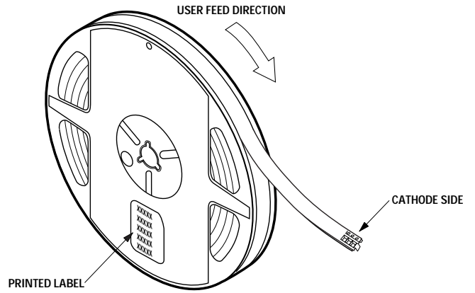
Figure 10. Reeling orientation.
