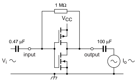
Fig 8. Test set-up for measuring forward transconductance
