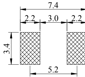
( PCB Pattern )
