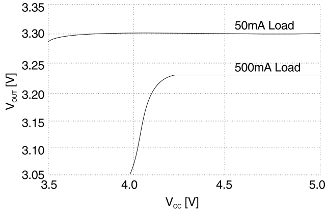
Figure 1. Dropout Characteristics
