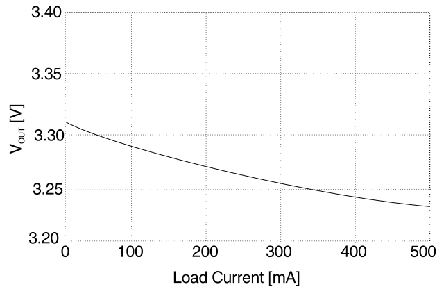
Figure 2. Load Regulation
