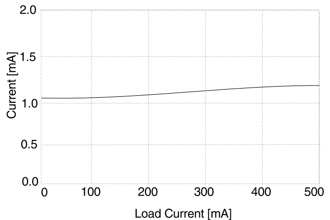
Figure 3. Ground Current
