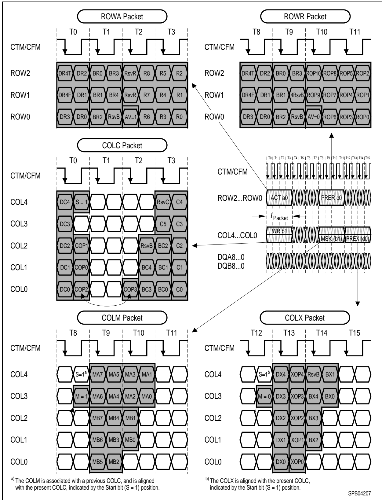
Figure 3 Packet Formats
