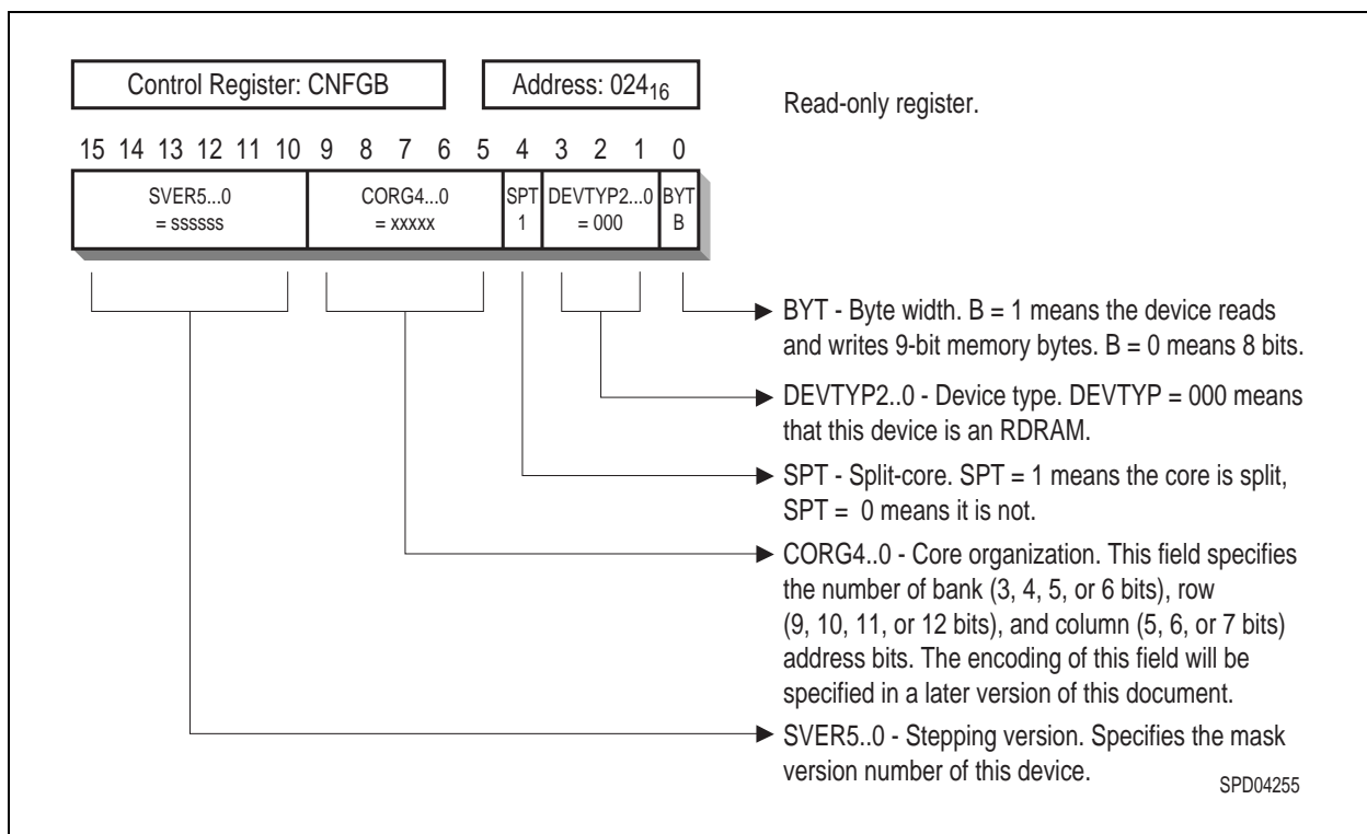
Figure 29 CNFGB Register
