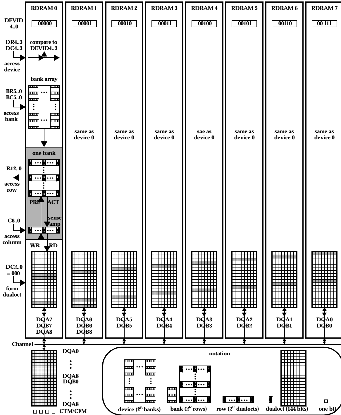
Figure 62: ACT, PRE, RD and WR Commands for Eight RDRAM System with IDM=1
