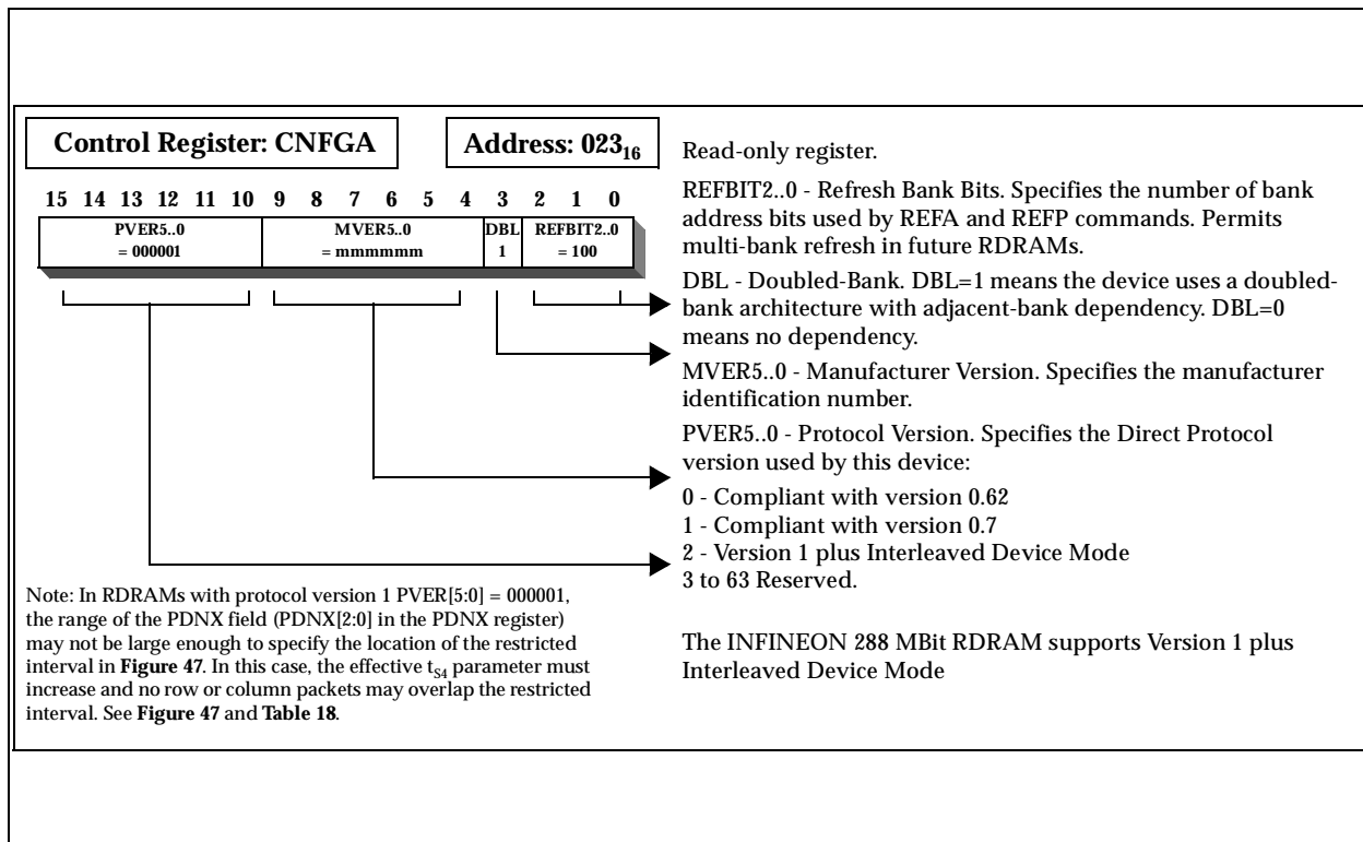
Figure 28 CNFGA Register
