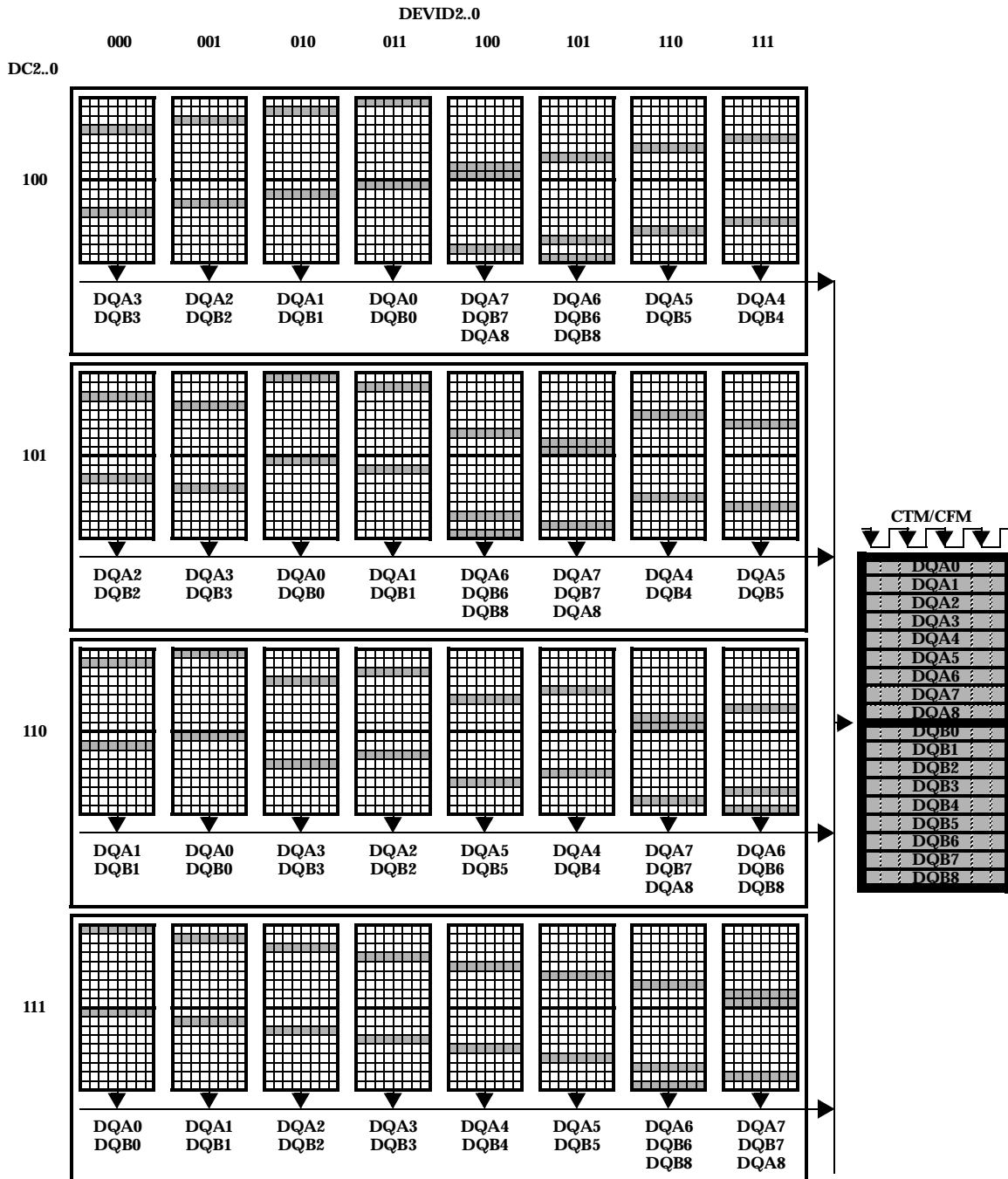
Figure 65: Mapping from DEVID2..0 and DC2..0 Fields to DQ Packet with IDM=1 (continued)
