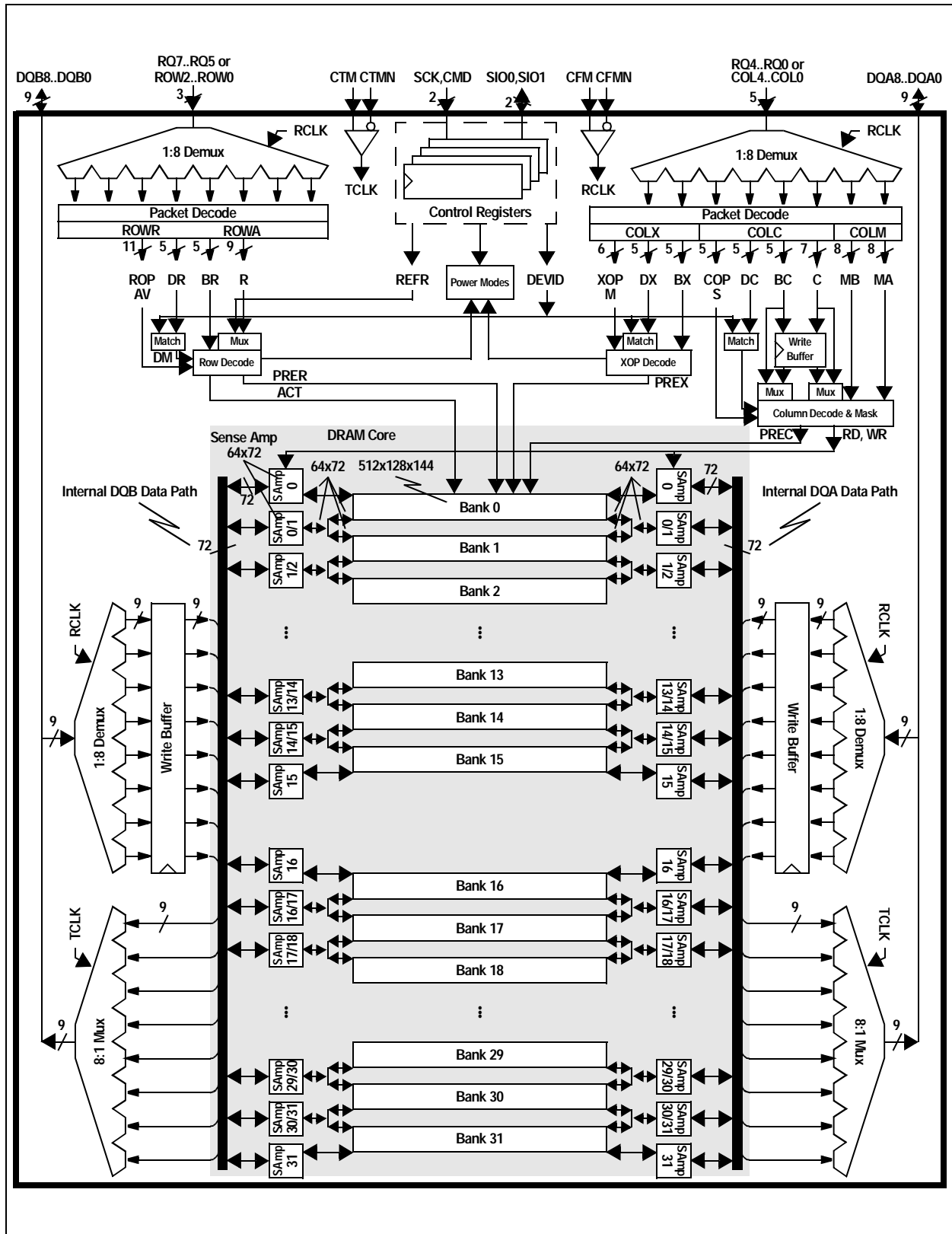
Figure 2 288-MBit Direct RDRAM Block Diagram
