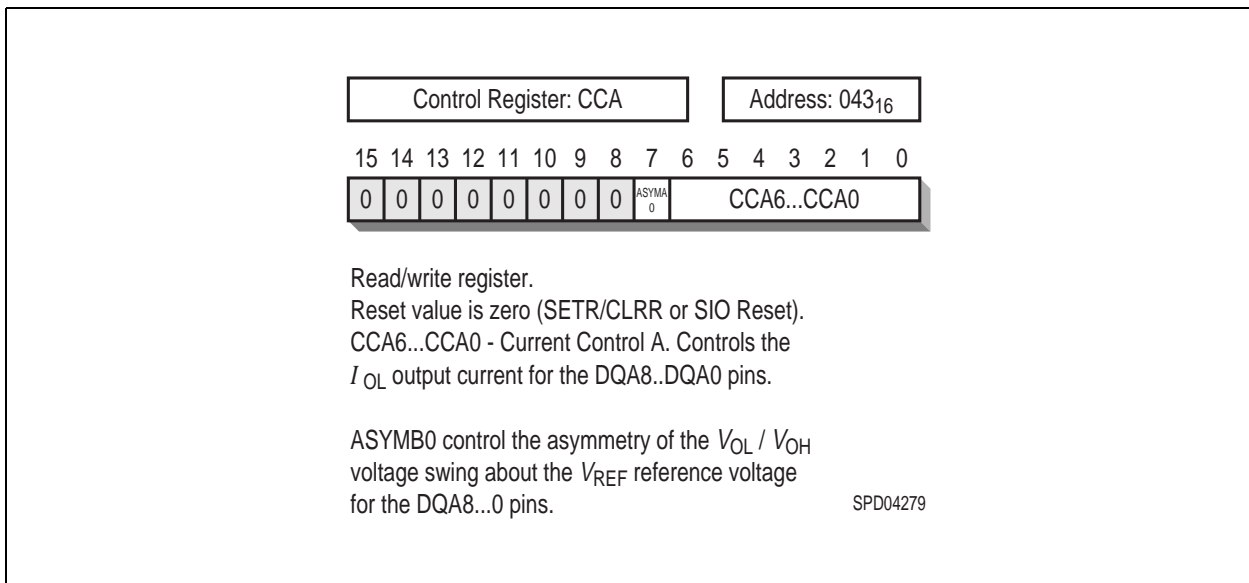
Figure 33 CCA Register
