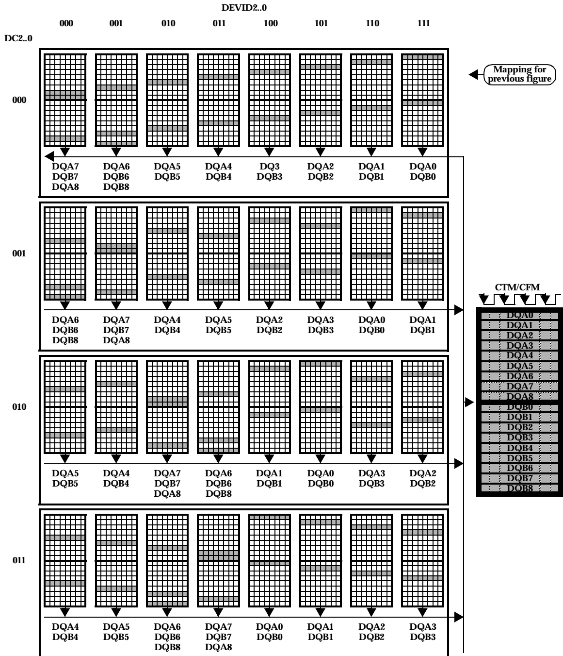
Figure 63: Mapping from DEVID2..0 and DC2..0 Fields to DQ Packet with IDM=1
