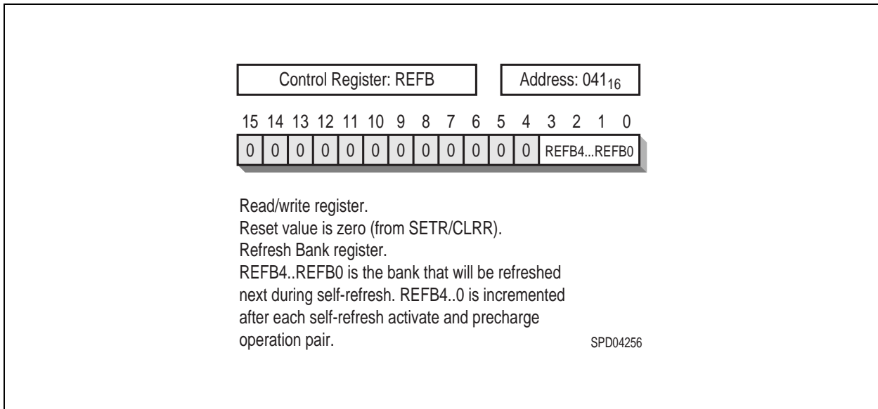
Figure 32 REFB Register
