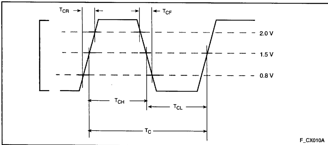
Figure 9. CLKIN Waveform
