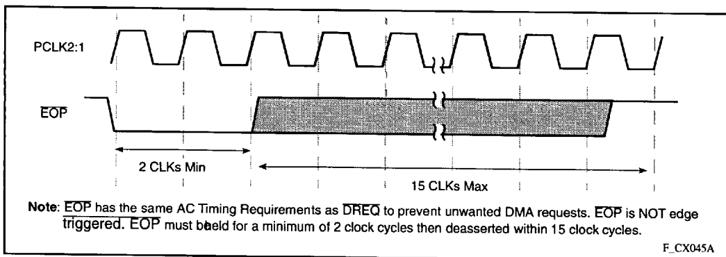
Figure 45. EOP Functional Timing
