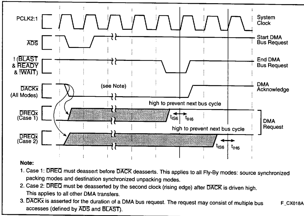
Figure 44. DREQ and DACK Functional Timing
