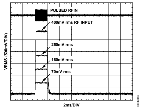
Figure 46. Output Response to Various RF Input Pulse Levels, Supply 3 V, Frequency 900 MHz, Square-Domain Filter Open, Output Filter 0.1 μF with Parallel 1 kΩ
