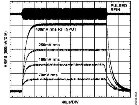
Figure 32. Output Response to Various RF Input Pulse Levels, Supply 3 V, Frequency 900 MHz, C_{FLTR} = 1 \text{ nF} , C_{OUT} = \text{Open} , R_{OUT} = \text{Open}
