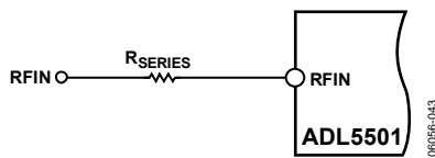
Figure 43. Attenuating the Input Signal
