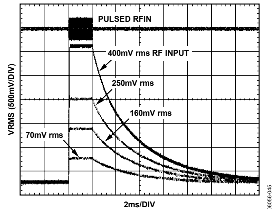
Figure 45. Output Response to Various RF Input Pulse Levels, Supply 3 V, Frequency 900 MHz, Square-Domain Filter Open, Output Filter 0.1 μF
