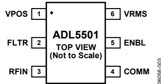
Figure 3. Pin Configuration
