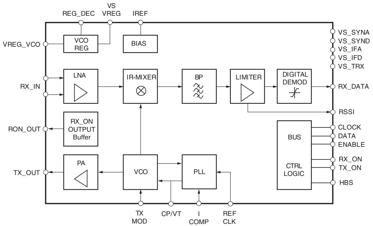
Figure 1-1. Block Diagram
