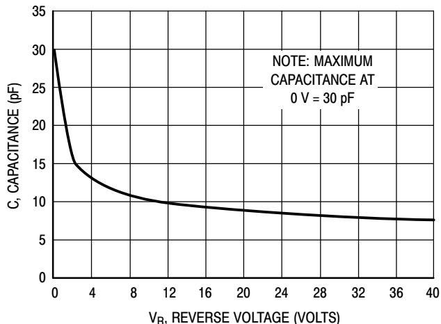
Figure 6. Maximum Capacitance
