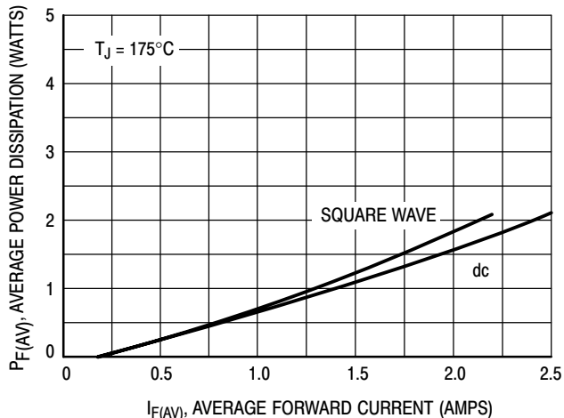
Figure 8. Power Dissipation
