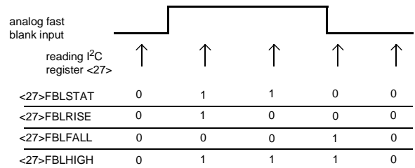
Fig. 2–11: Fast Blank Monitor
