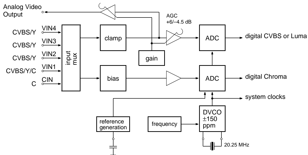
Fig. 2–1: Analog front-end
