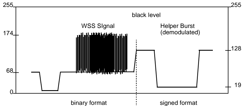
Fig. 2–17: PAL+ helper reference line output signal
