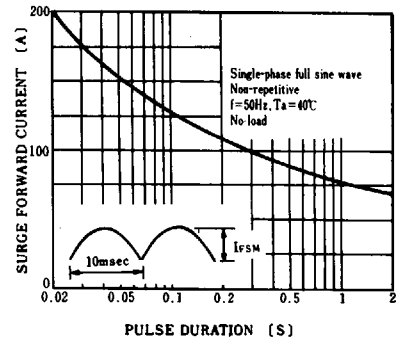
FIG.6-SURGE CURRENT RATINGS
