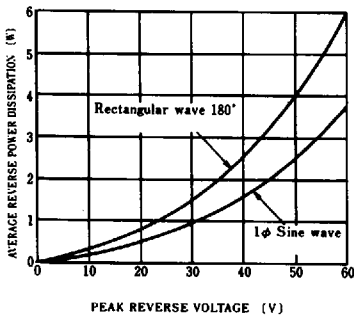
FIG.4-AVERAGE REVERSE POWER DISSIPATION
