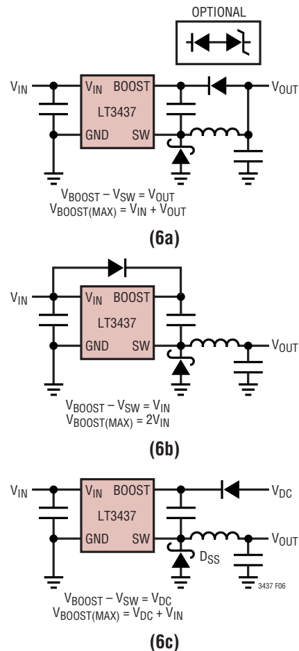
Figure 6. BOOST Pin Configurations
