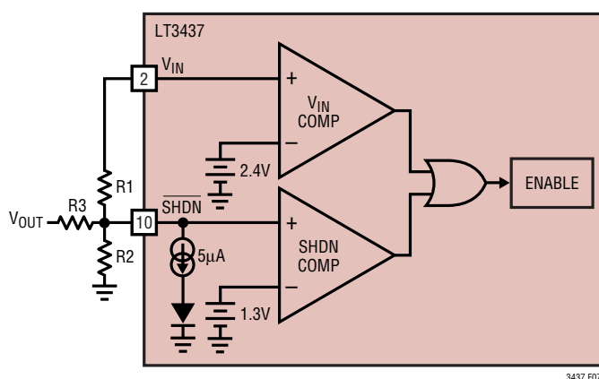
Figure 7. Undervoltage Lockout
