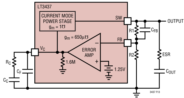
Figure 10. Model for Loop Response
