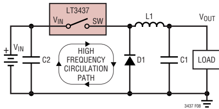
Figure 8. High Speed Switching Path
