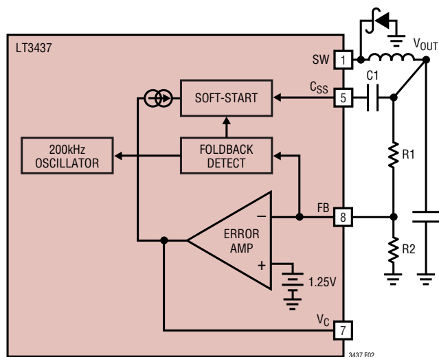
Figure 2. Feedback Network
