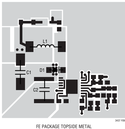
FE PACKAGE TOPSIDE METAL
