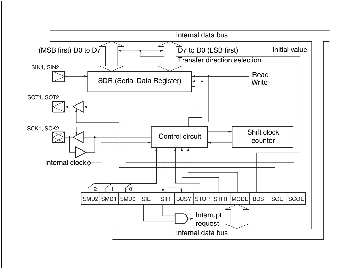
(2) Block Diagram
