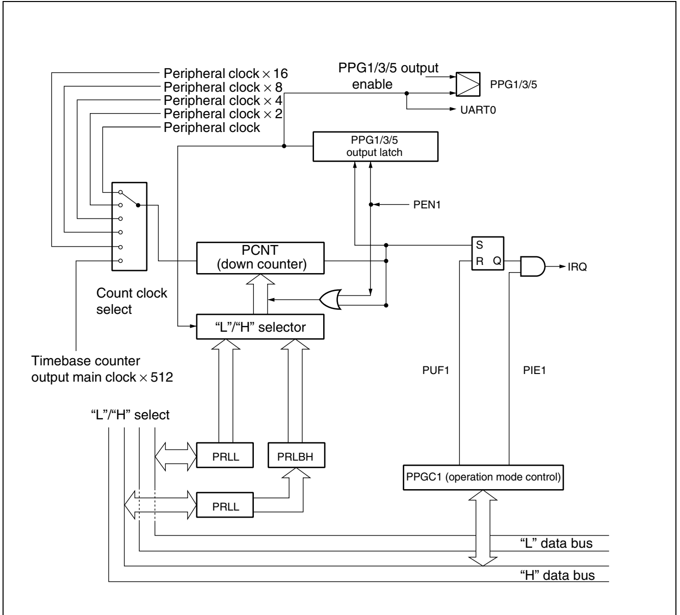
• 8-bit PPG ch.1/3/5 Block Diagram
