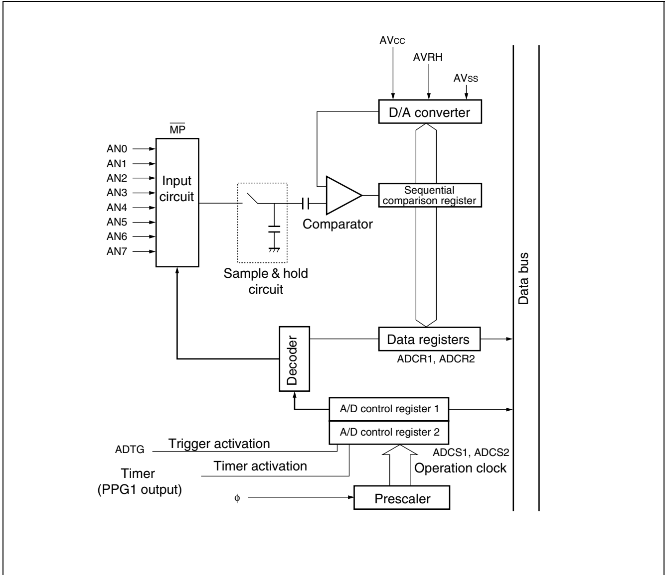
(2) Block Diagram
