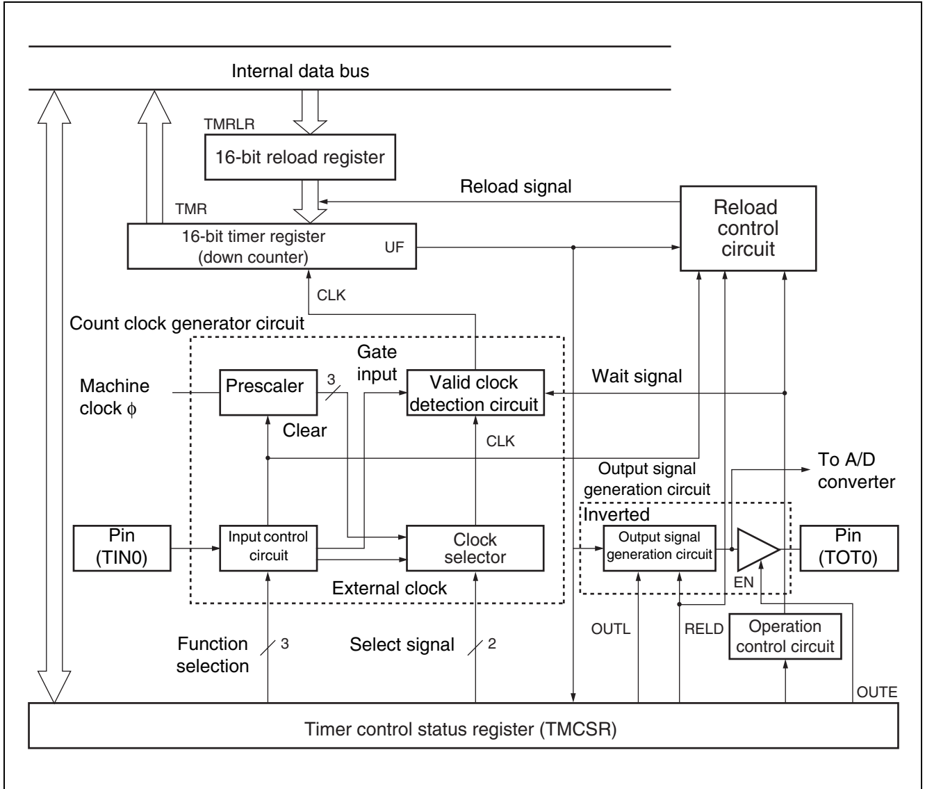
(2) Block Diagram
