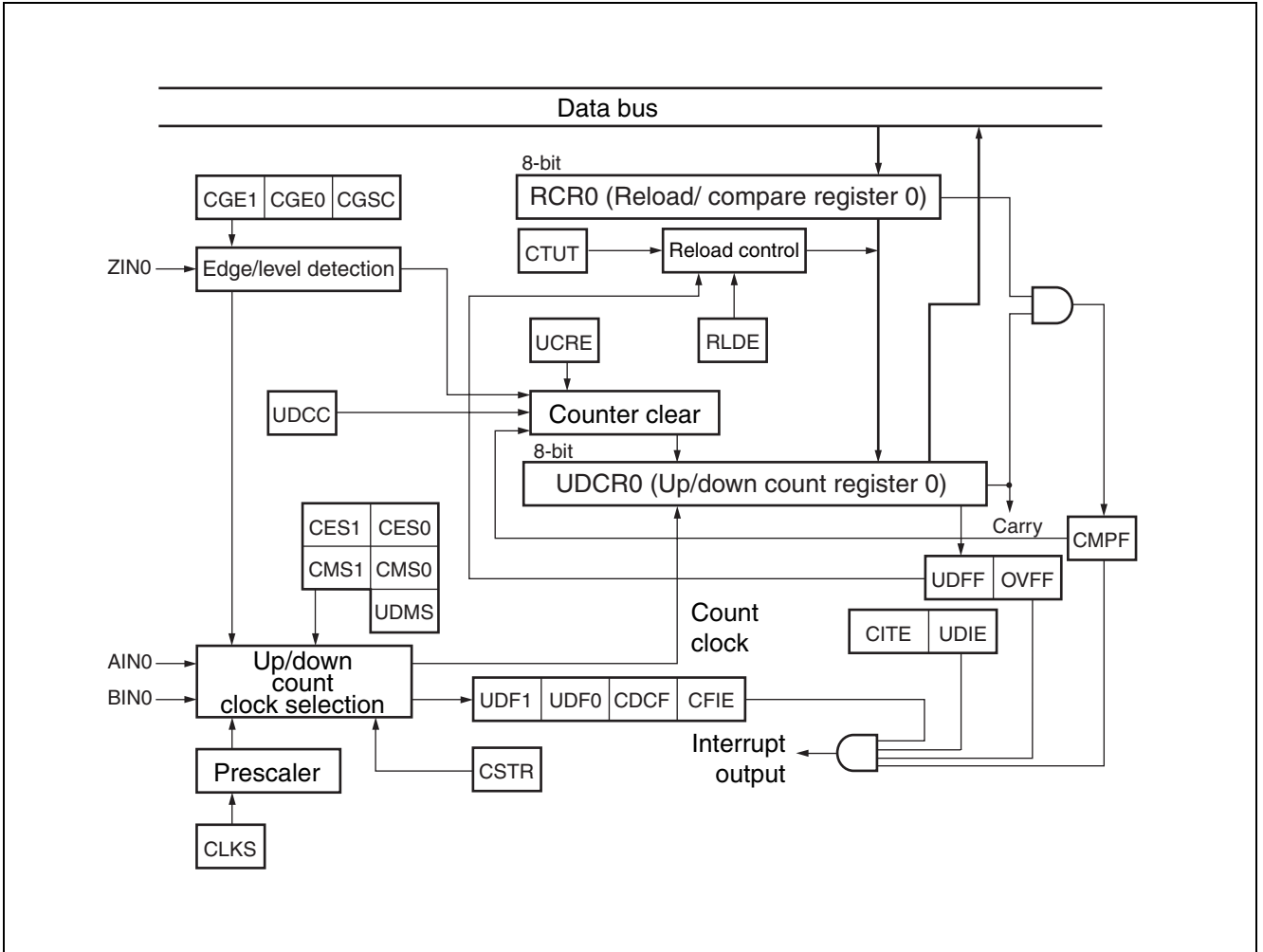
(3) Block Diagram
