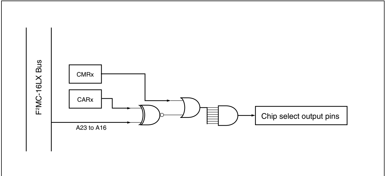
(2) Block Diagram
