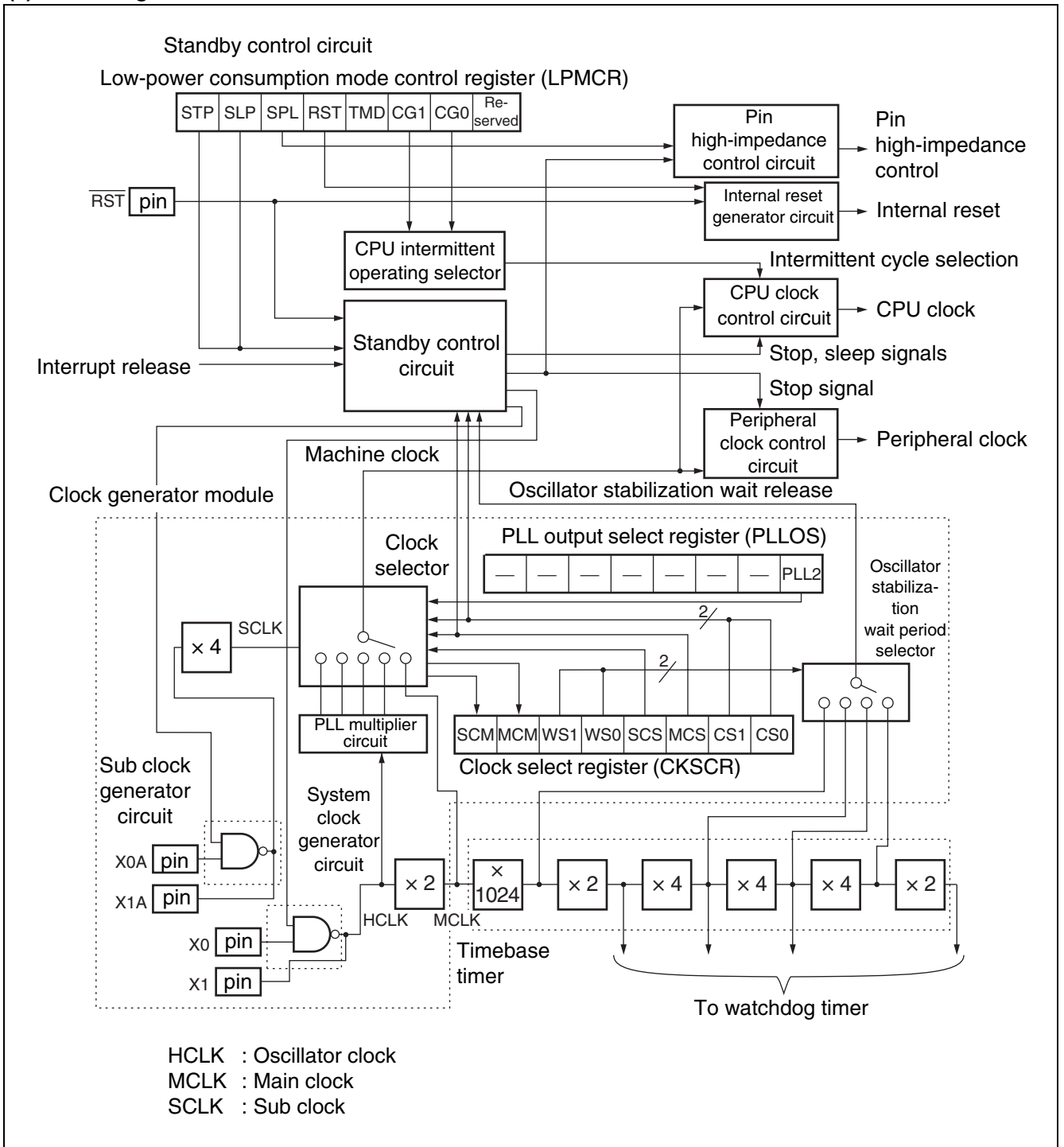
(2) Block Diagram
