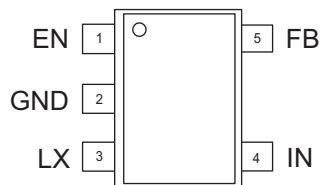
Adjustable Output Version (AAT1106ICB-0.6)
