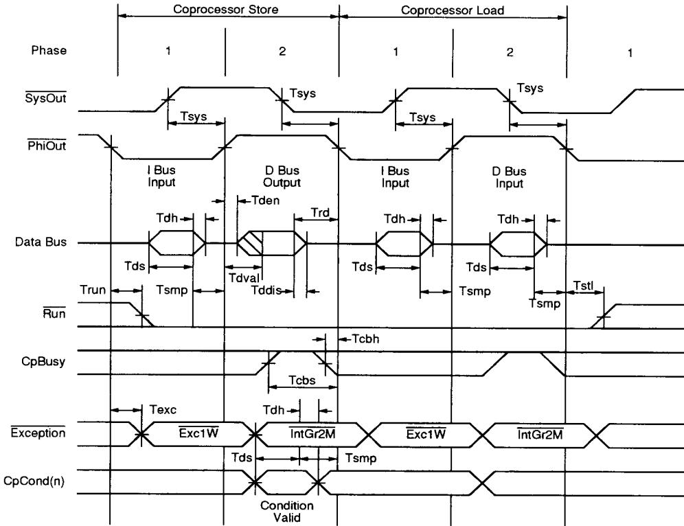
Figure 20. Coprocessor Load/Store Timing
