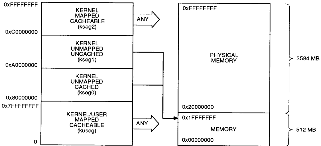
Figure 7. IDT79R3500 Virtual Address Mapping
