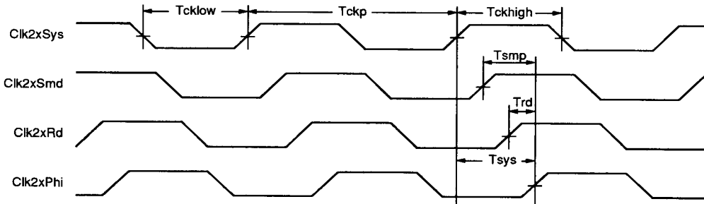
Figure 15. Input Clock Timing
