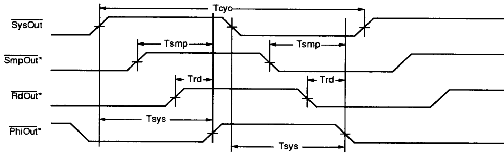
Figure 16. Processor Reference Clock Timing
