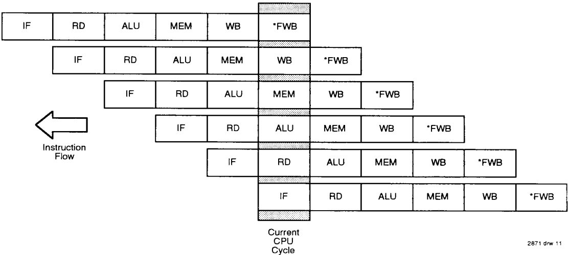
Figure 11. IDT79R3500 Execution Sequence
