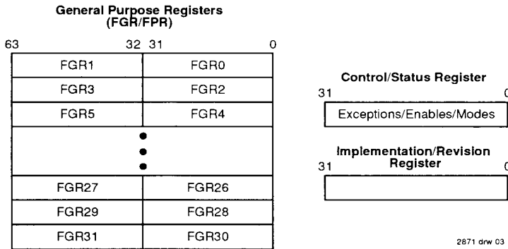
Figure 3. FPA Registers
