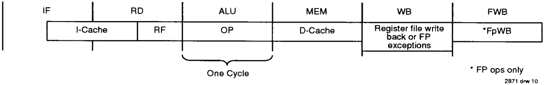
Figure 10. Instruction Execution
