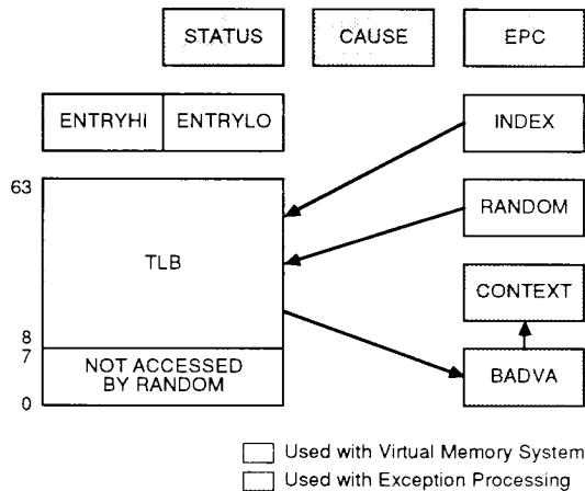
Figure 5. The System Coprocessor Registers
