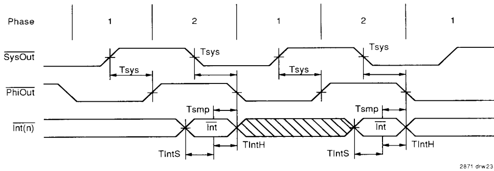
Figure 21. Interrupt Timing
