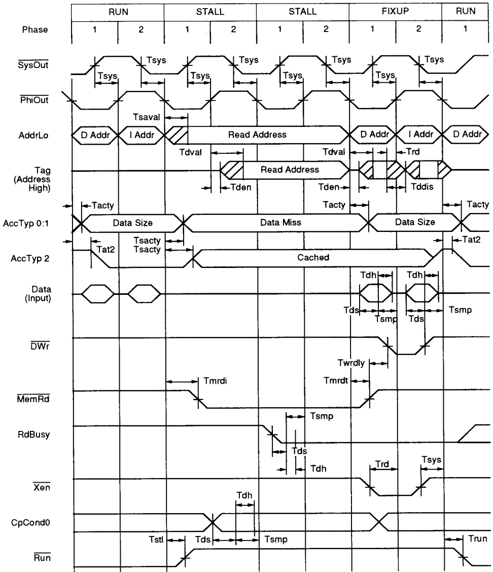
Figure 19. Memory Read Timing
