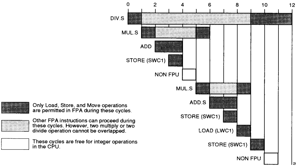
Figure 9. Examples of Overlapping Floating Point Operation
