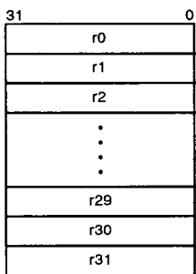
Figure 2. IDT79R3500 CPU Registers
