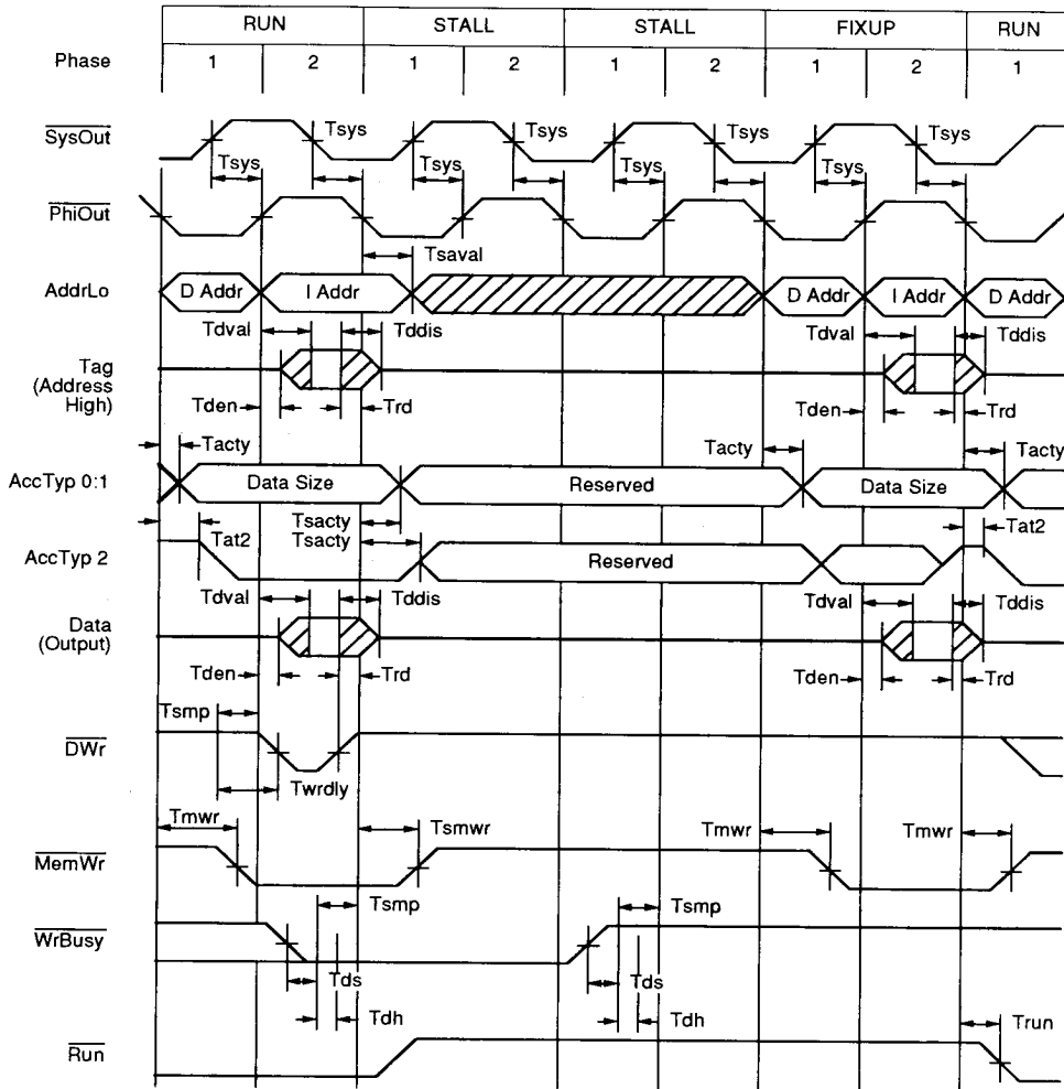
Figure 18. Memory Write Timing
