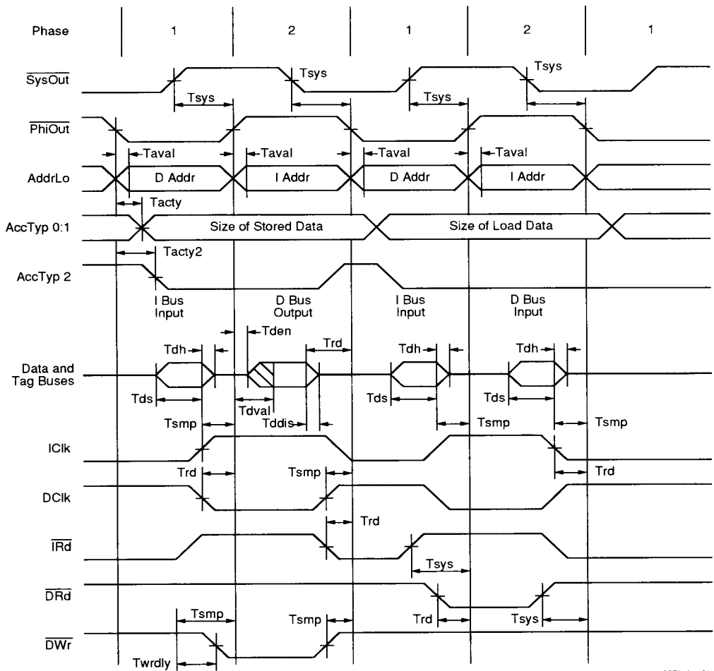
Figure 17. Synchronous Memory (Cache) Timing
