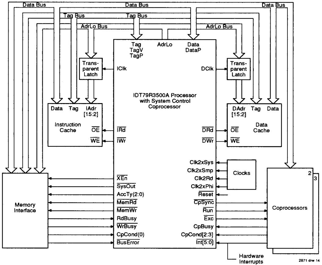
Figure 14. IDT79R3500 Subsystem Interfaces Example; 64 KB Caches
