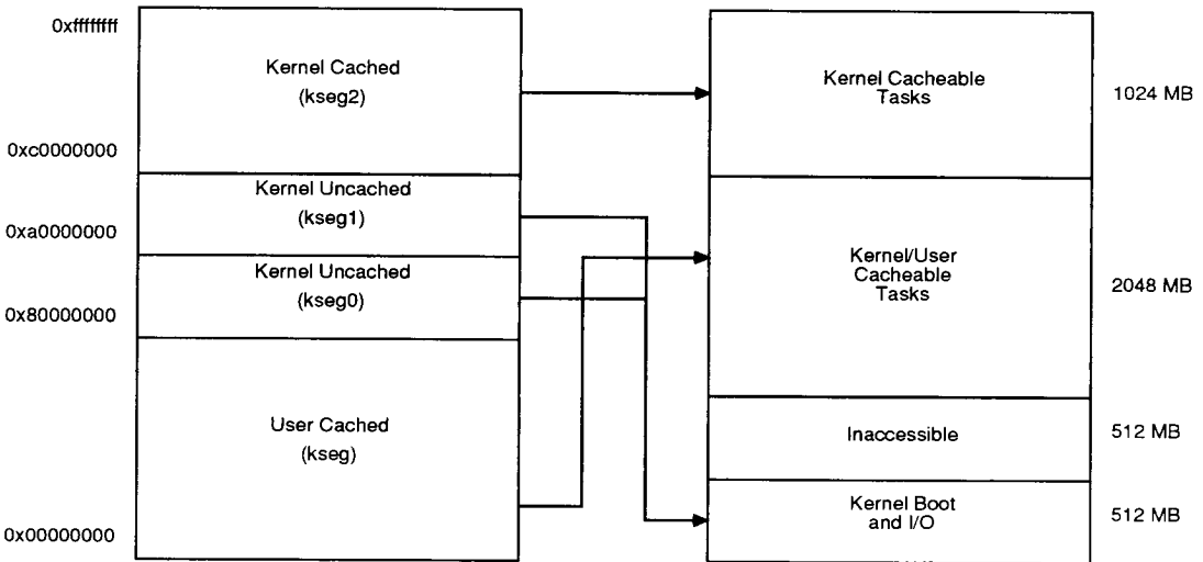
Figure 8. TLB Disabled Mapping
