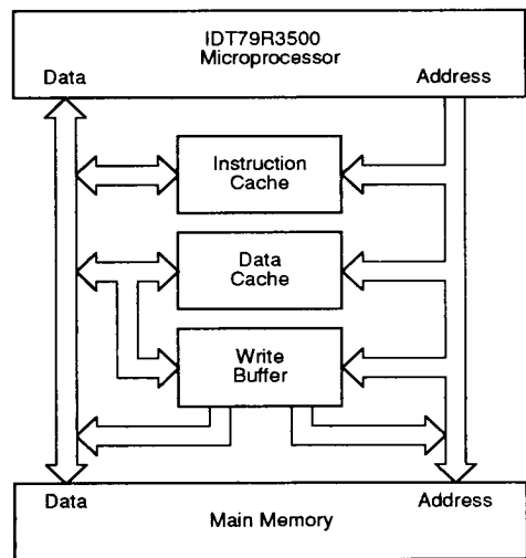
Figure 13. An IDT79R3500 System with a High-Performance Memory System
