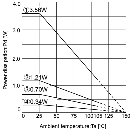
Fig.26 Thermal derating curve (VQFN020V4040)
