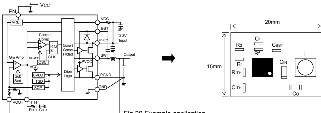
Fig.20 Example application
