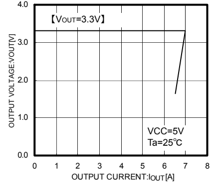
Fig.5 I OUT - V OUT
