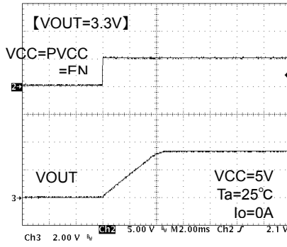
Fig.13 Soft start waveform
