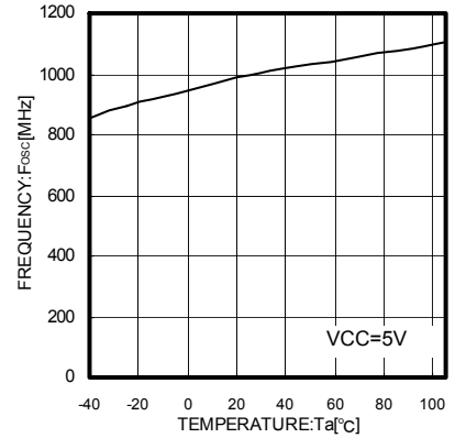
Fig.8 T a - F osc
