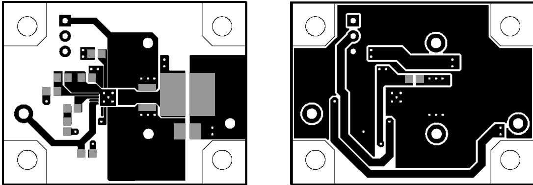
Fig.33 Layout diagram
