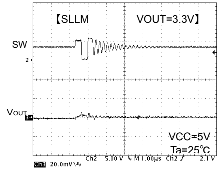
Fig.14 SW waveform Io=10mA
