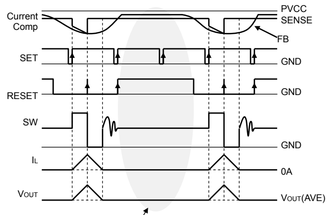
Fig.23 SLLM™ switching timing chart
