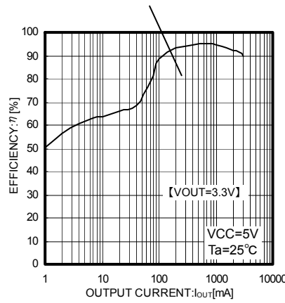
Fig.7 Efficiency
