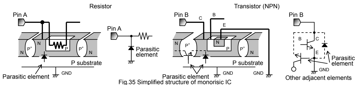
Fig.35 Simplified structure of monolithic IC
