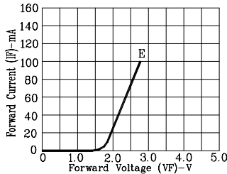
Fig3. FORWARD CURRENT VS. FORWARD VOLTAGE
