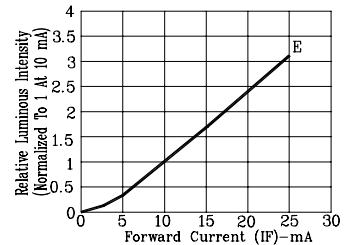
Fig4. RELATIVE LUMINOUS INTENSITY VS. FORWARD CURRENT
