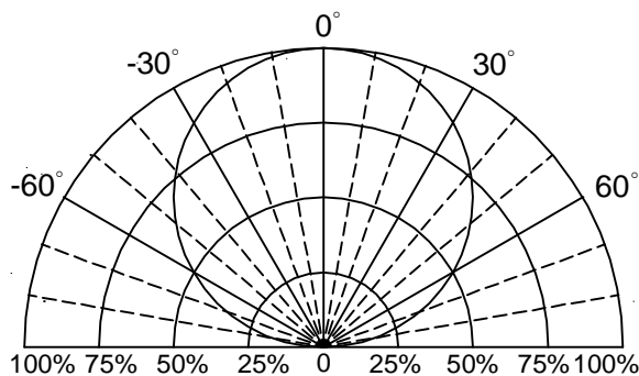
Fig.6 Directive Radiation
