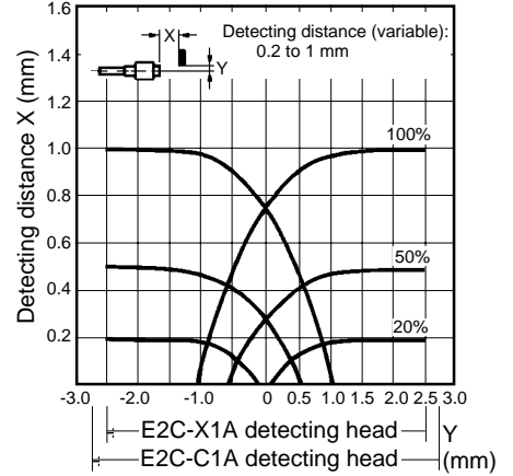
Shielded M5 and 5.4 mm dia. sensors E2C-X1A, E2C-C1A
