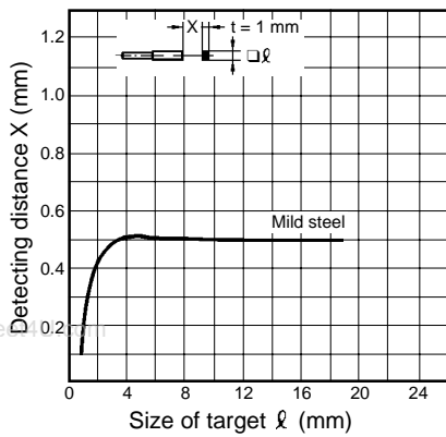
Shielded M8 sensor E2C-X1R5A
