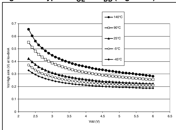
Figure 84. Typical V_{OL} vs V_{DD} (Port C)
