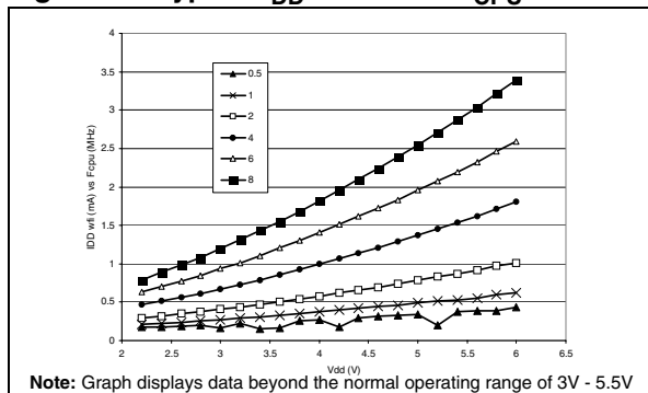
Figure 71. Typical I_{DD} in WAIT at f_{CPU} = 8 MHz
