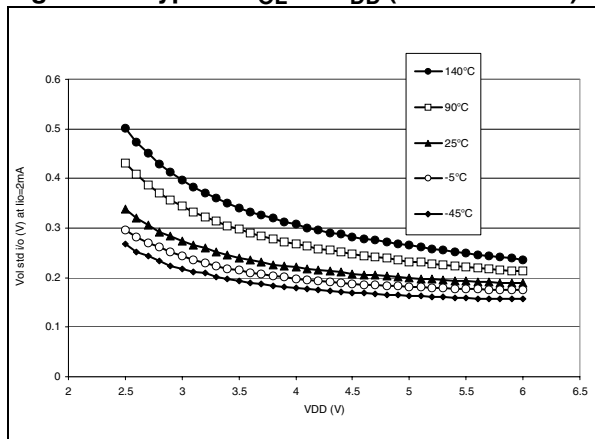
Figure 83. Typical V_{OL} vs V_{DD} (High-sink)
