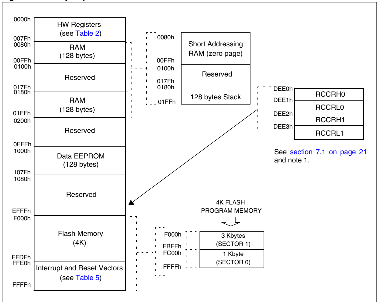
Figure 3. Memory Map
