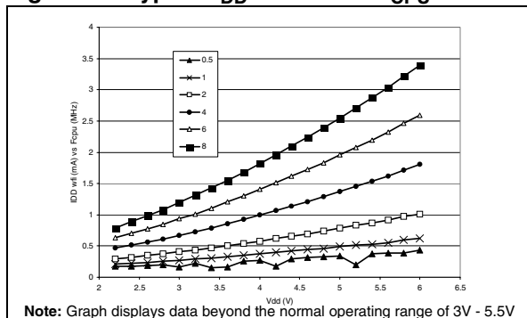
Figure 70. Typical I_{DD} in WAIT vs f_{CPU}
