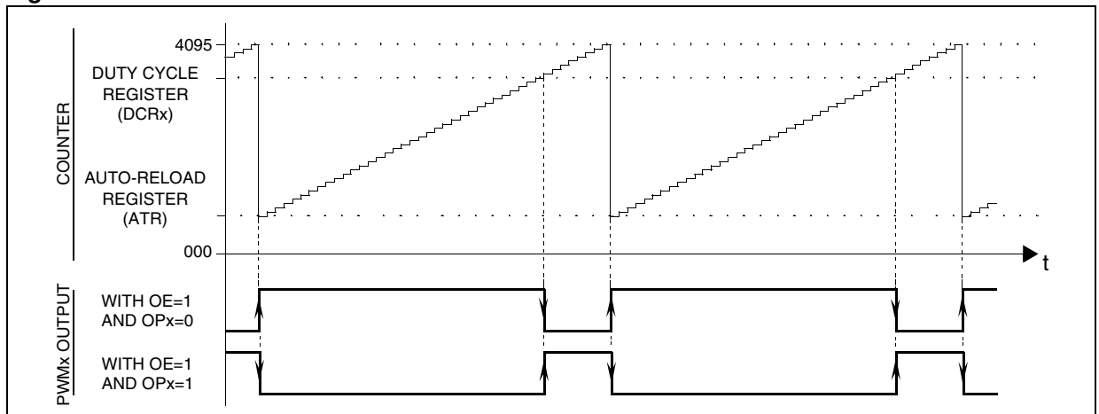
Figure 35. PWM Function
