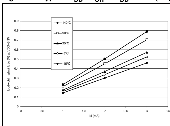
Figure 87. Typical V_{DD} - V_{OH} at V_{DD} = 3.3V (HS)
