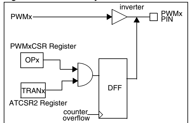
Figure 34. PWM Polarity Inversion
