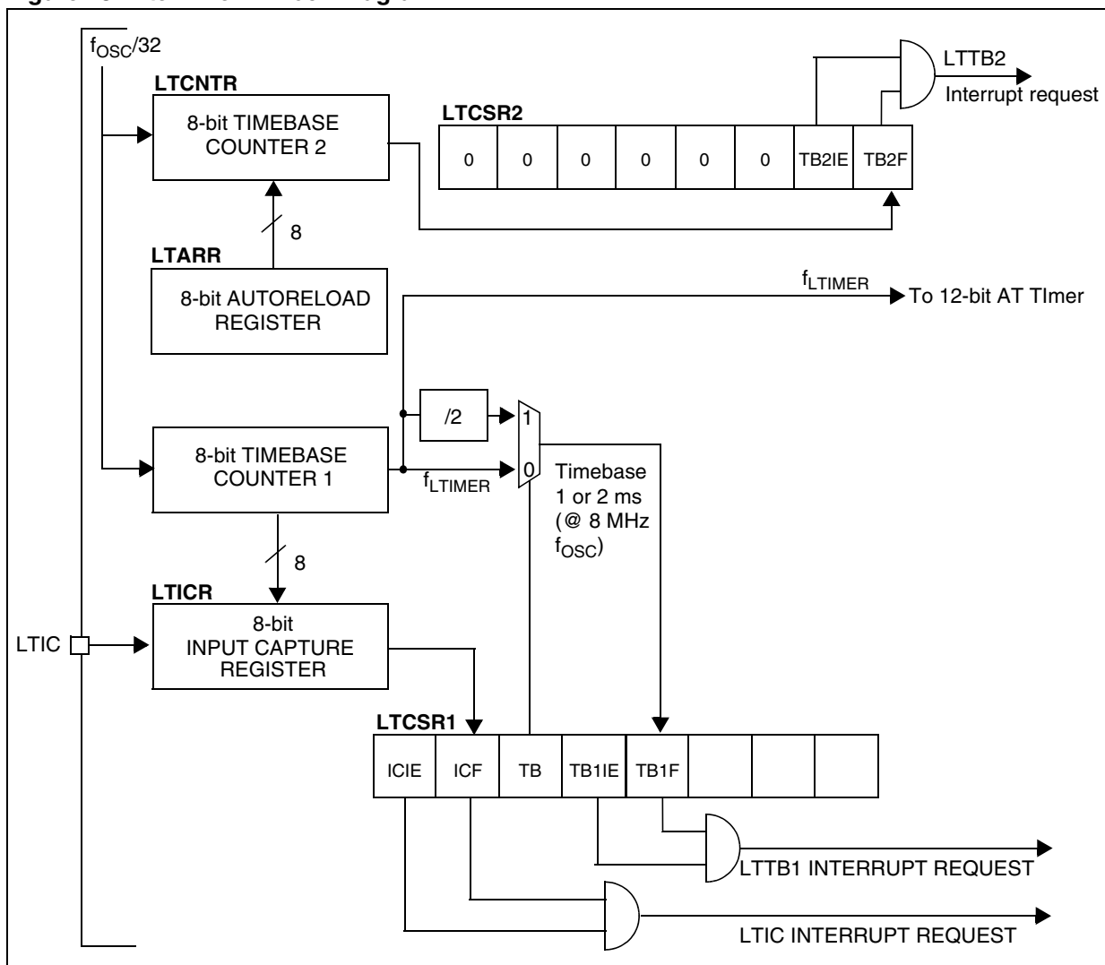
Figure 48. Lite Timer 2 Block Diagram
