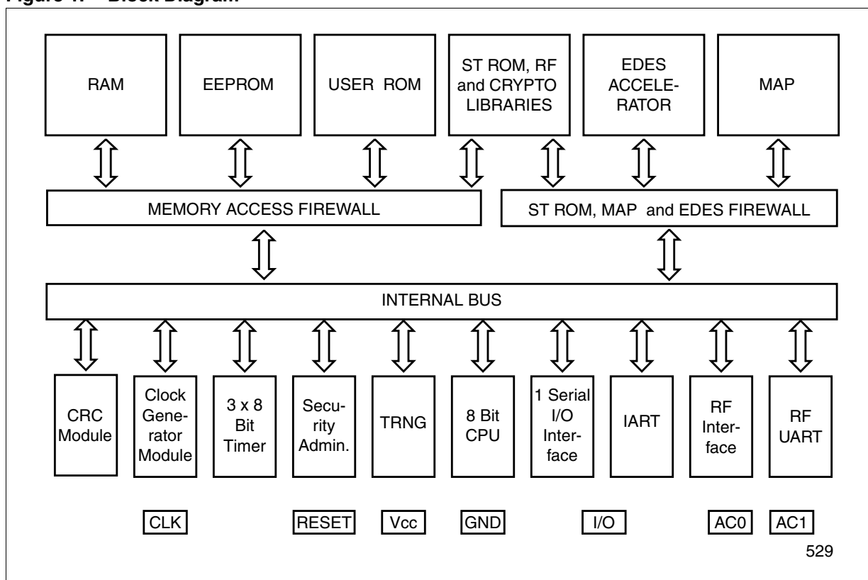
Figure 1. Block Diagram
