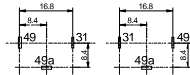
Mounting (Bottom views)
