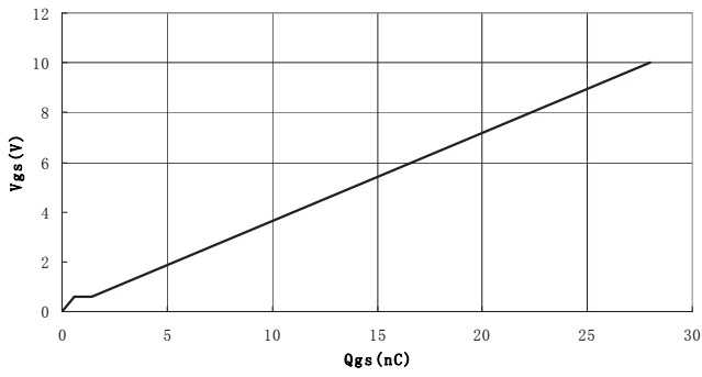
Figure 5. Gate Charge
