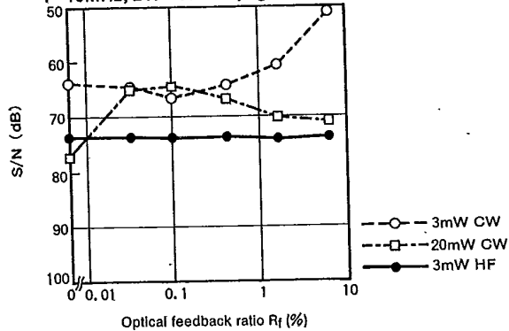
Fig. 14 S/N vs. optical feedback ratio
