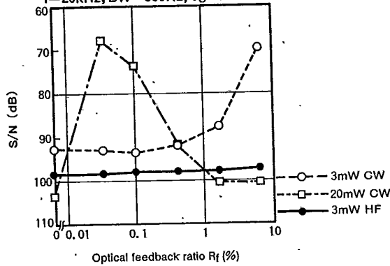
Fig. 13 S/N vs. optical feedback ratio
