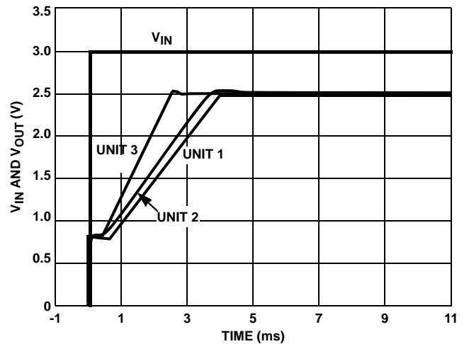
FIGURE 119. TURN-ON TIME
