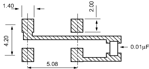
Figure 2) Land Pattern
