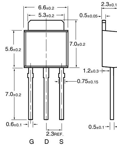
TO-251
