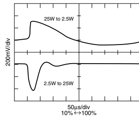
MTR2805S STEP LOAD RESPONSE
