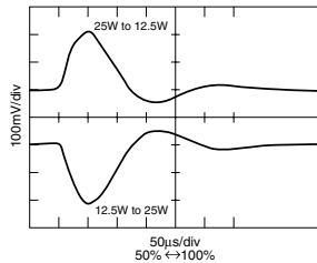
MTR2805S STEP LOAD RESPONSE
