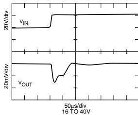
MTR2805S STEP LINE RESPONSE
