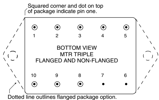
FIGURE 5: PIN OUT TRIPLE OUTPUT MODELS
