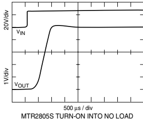
MTR2805S TURN-ON INTO NO LOAD
