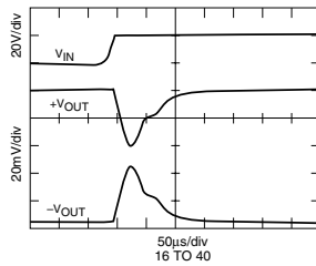
MTR2815D STEP LINE RESPONSE
