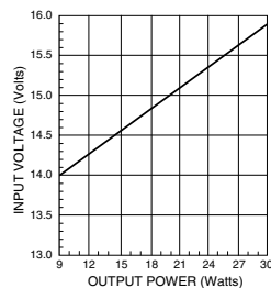
1% DROP MTR SINGLES AND DUALS LOW LINE DROPOUT
