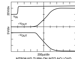
MTR2815D TURN-ON INTO NO LOAD
