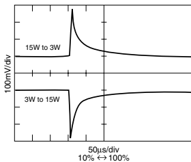
MTR2815D +VOUT STEP LOAD RESPONSE
