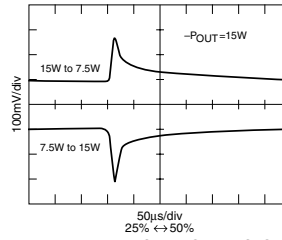
MTR2815D +VOUT STEP LOAD RESPONSE
