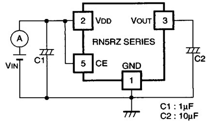
Fig.2 Supply Current Test Circuit
