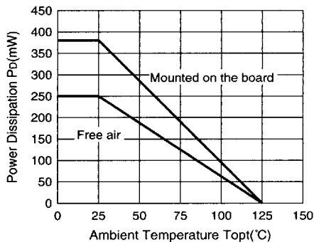
RN5RZ30B(SOT-23-5)
