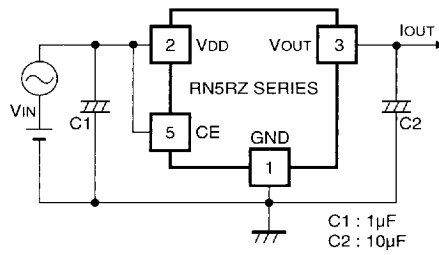
Fig.5 Ripple Rejection Test Circuit
