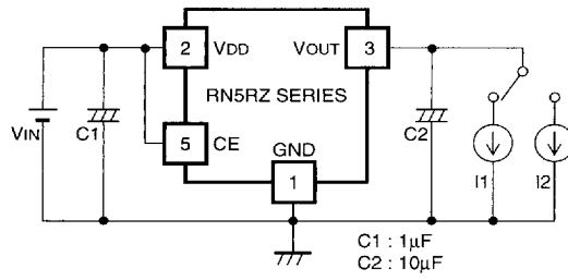
Fig.4 Load Transient Response Test Circuit
