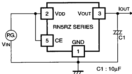
Fig.3 Line Transient Response Test Circuit
