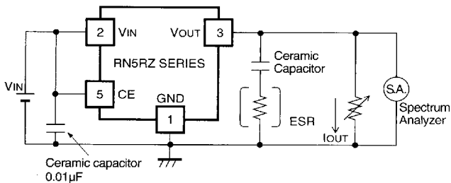
Measuring circuit for white noise ; RN5RZ30B
