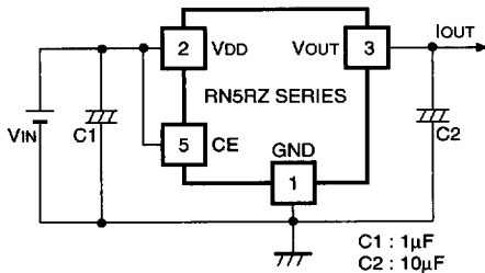
Fig.1 Standard Test Circuit
