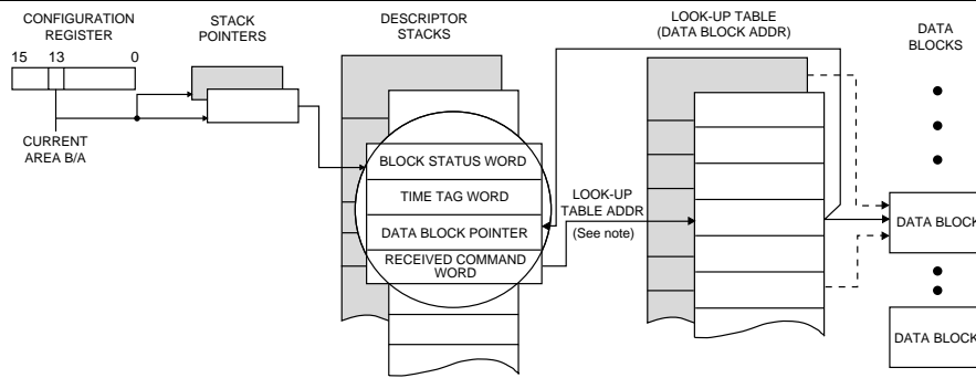
FIGURE 5. RT MEMORY MANAGEMENT: SINGLE MESSAGE MODE
