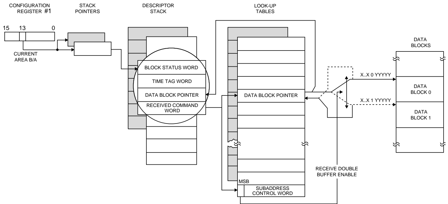
FIGURE 7. RT MEMORY MANAGEMENT: SUBADDRESS DOUBLE BUFFERING MODE
