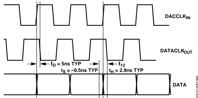
Figure 37. Data Timing, DLL Off, 1× Interpolation, DCLKPOL = 1
