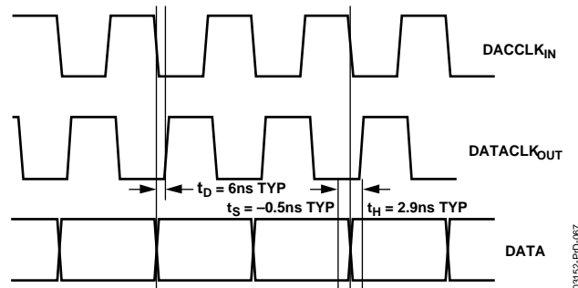
Figure 38. Data Timing, DLL Off, 1× Interpolation, DCLKPOL = 0
