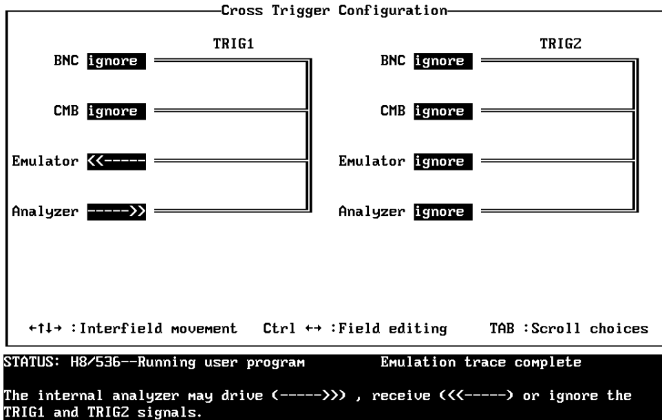
Figure 5-1. Cross Trigger Configuration
