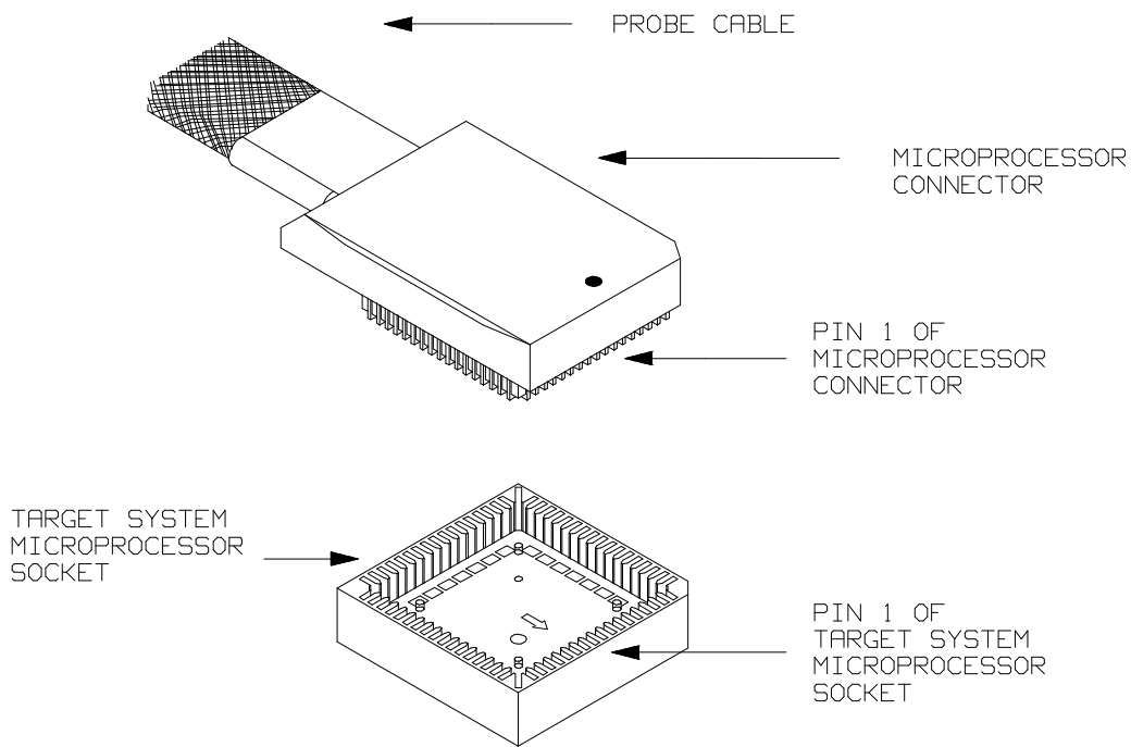
Figure 3-8. Installing into a PLCC type socket
