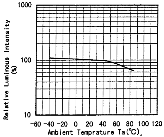
Relative Luminous Intensity vs. Ambient Temperature ( I_F=20\text{mA} )
