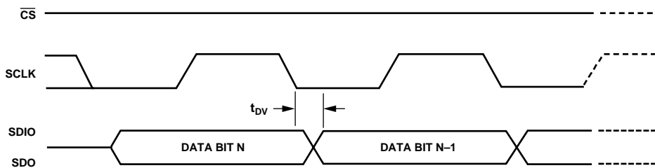
Figure 36. Timing Diagram for Register Read from AD9775
