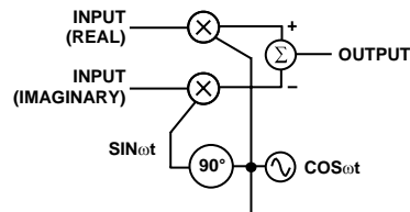
Figure 78. Quadrature Modulator
