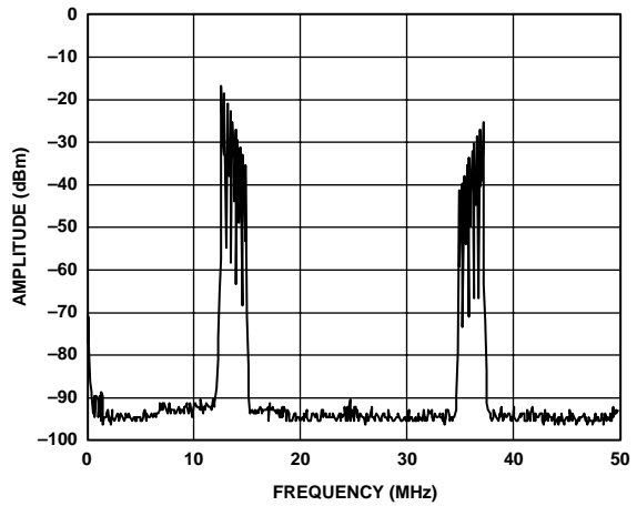
Figure 91. AD9775 Real DAC Output of Complex Input Signal Near Baseband (Positive Frequencies Only), Interpolation = 4x, Complex Modulation in AD9775 = +f_{DAC}/4
