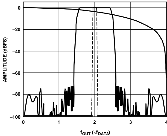
Figure 68. 4x Interpolation, Modulation = f_{DAC}/4
