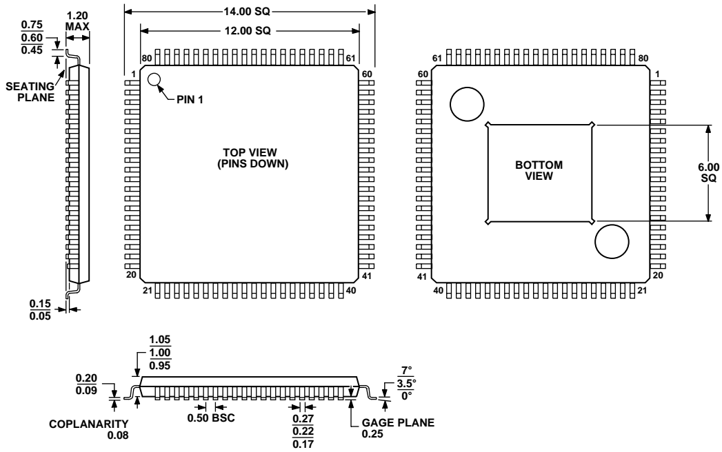
Figure 115. 80-Lead Thermally Enhanced, Thin Plastic Quad Flat Package [TQFP] (SV-80) Dimensions shown in millimeters
