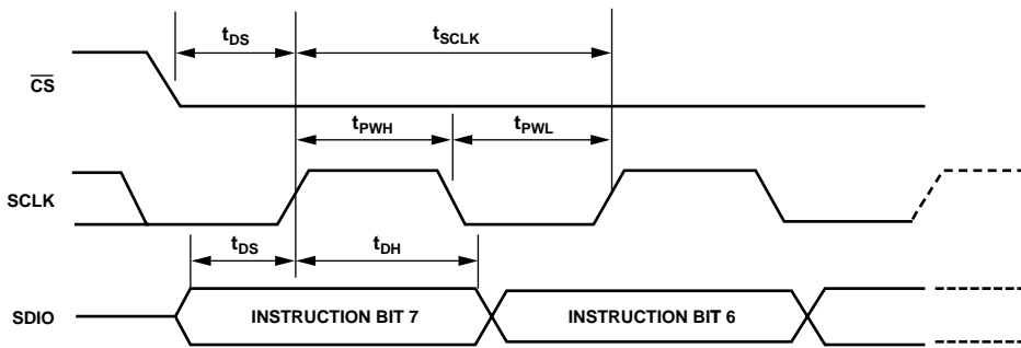
Figure 35. Timing Diagram for Register Write to AD9775
