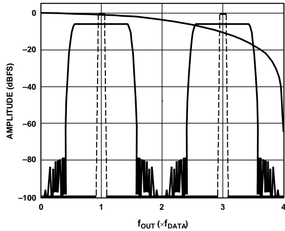
Figure 69. 4x Interpolation, Modulation = f_{DAC}/2
