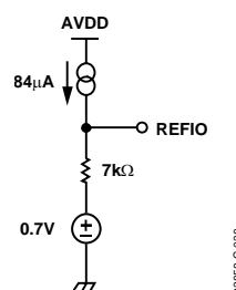
Figure 38. Equivalent Internal Reference Circuit
