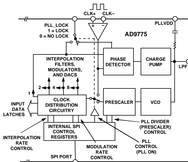
Figure 45. PLL and Clock Circuitry with PLL Enabled
