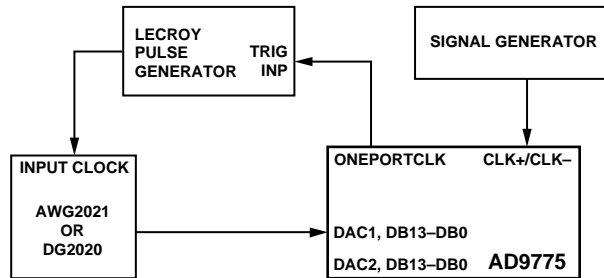
JUMPER CONFIGURATION FOR ONE PORT MODE PLL ON
