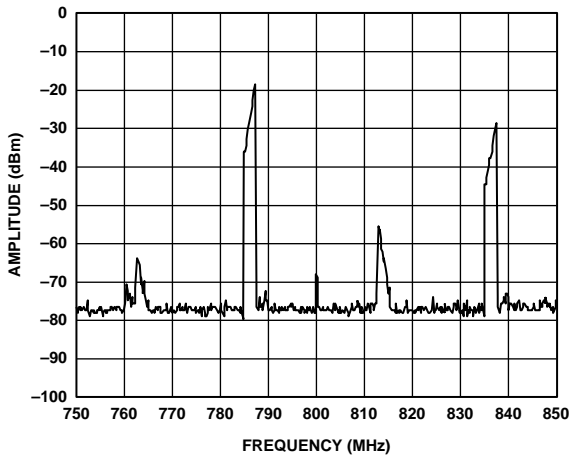
Figure 94. AD9775 Complex Output from Figure 93, Now Quadrature Modulated by AD8345 (LO = 800 MHz)
