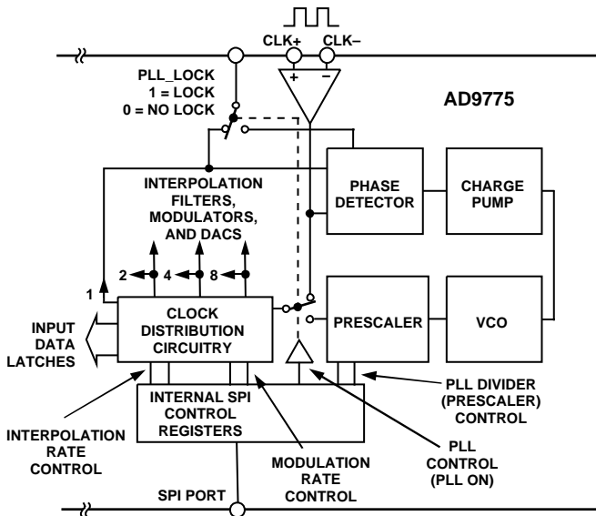
Figure 46. PLL and Clock Circuitry with PLL Disabled
