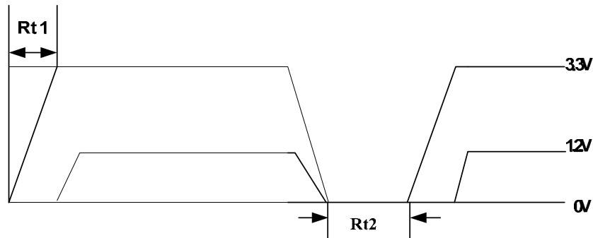
Figure 19. Power Sequence
