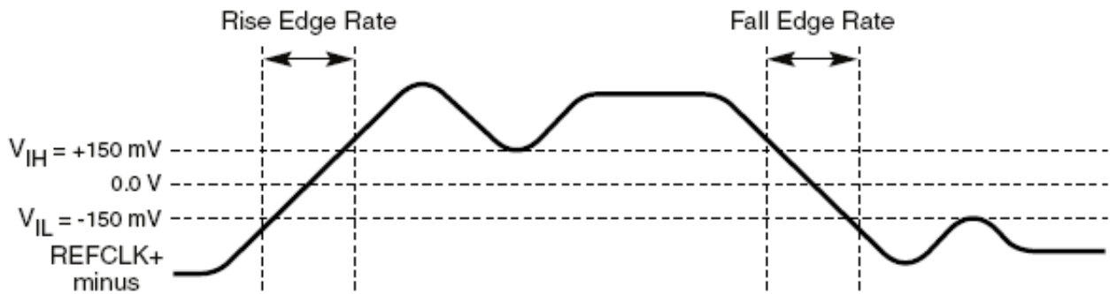
Figure 25. Differential Measurement Points for Rise and Fall Time
