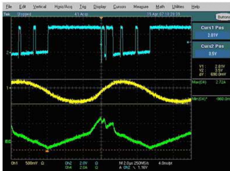
Figure 14. Ceramic 22µF 0805 (Y5V) (Bad)
