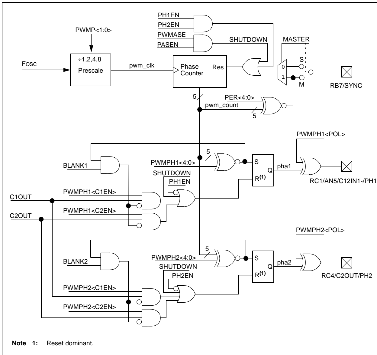
FIGURE 13-1: TWO-PHASE PWM SIMPLIFIED BLOCK DIAGRAM
