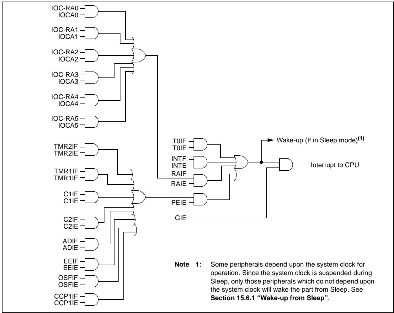
FIGURE 15-6: INTERRUPT LOGIC
