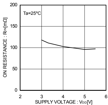
Fig.7 ON resistance
