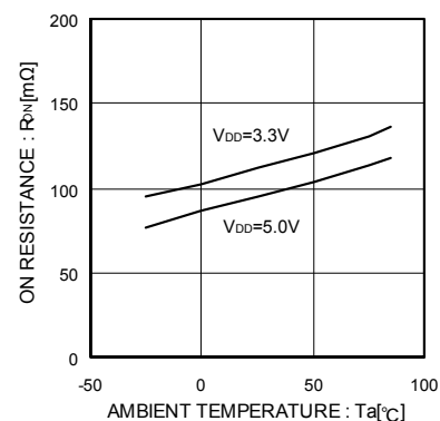
Fig.8 ON resistance
