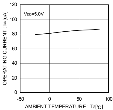
Fig.4 Operating current
