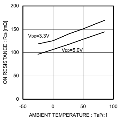
Fig.32 ON resistance
