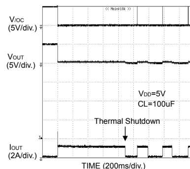
Fig.82 Over current response Output shortcircuit at Enable (BD2052AFJ)
