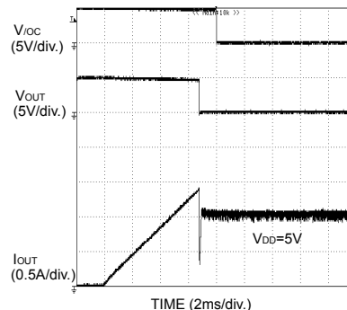
Fig.76 Over current response Ramped load (BD2052AFJ)
