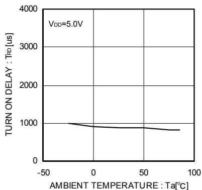
Fig.12 Output rise delay time
