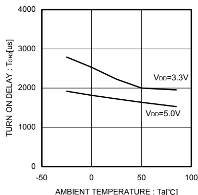
Fig.36 Output rise delay time
