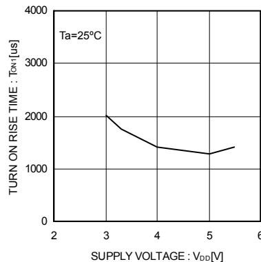
Fig.33 Output rise time
