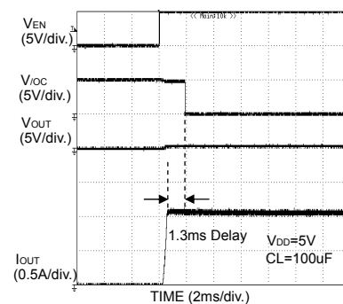
Fig.79 Over current response Enable to shortcircuit (BD2052AFJ)
