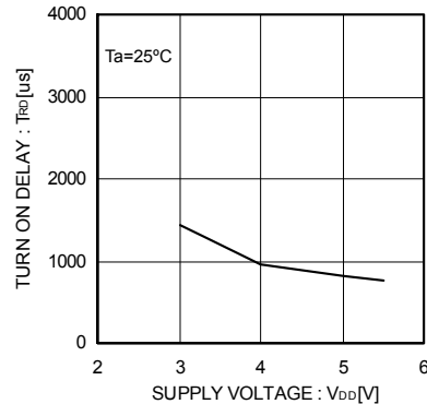
Fig.11 Output rise delay time
