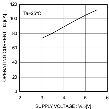
Fig.25 Operating current
