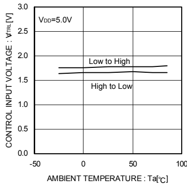
Fig.30 CTRL input voltage (BD6517F)
