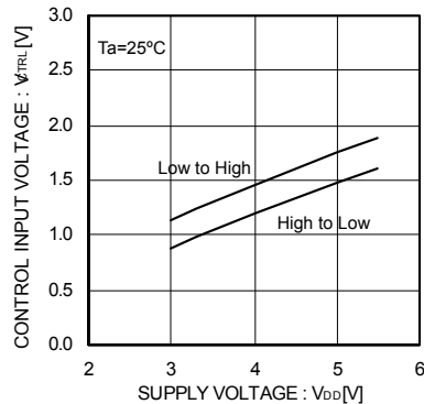
Fig.5 CTRL input voltage
