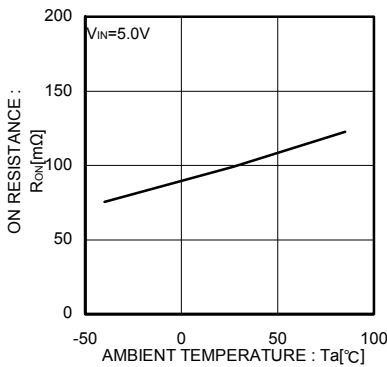
Fig.58 ON resistance
