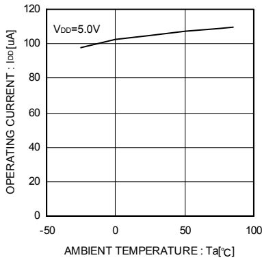
Fig.26 Operating current
