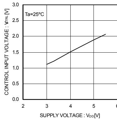
Fig.27 CTRL input voltage (BD6516F)
