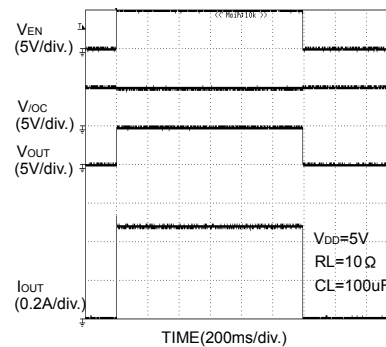
Fig.73 Output rise, fall characteristic (BD2052AFJ)
