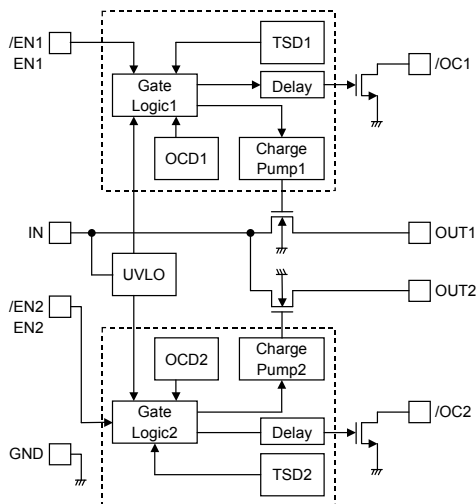
Fig.85 Block diagram
