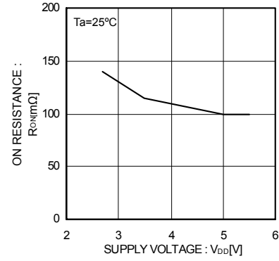
Fig.57 ON resistance
