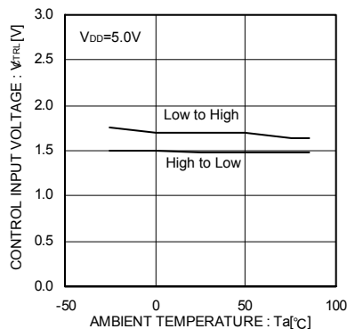
Fig.6 CTRL input voltage
