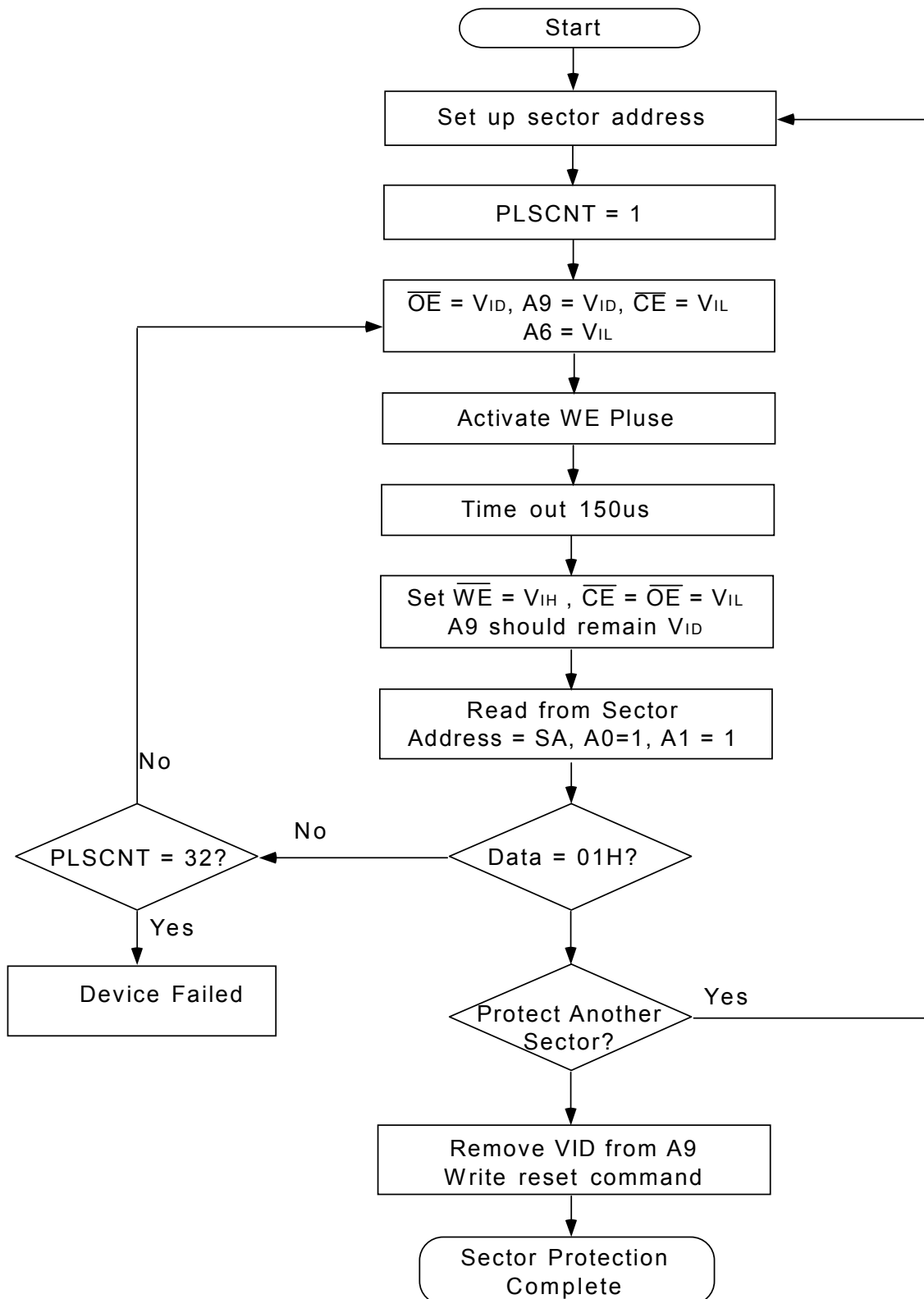
Figure 18. Sector Protection Algorithm (A9, \overline{OE} Control)
