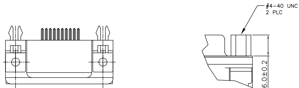
DETAIL Z (W/SCREWLOCKS OPTION)
